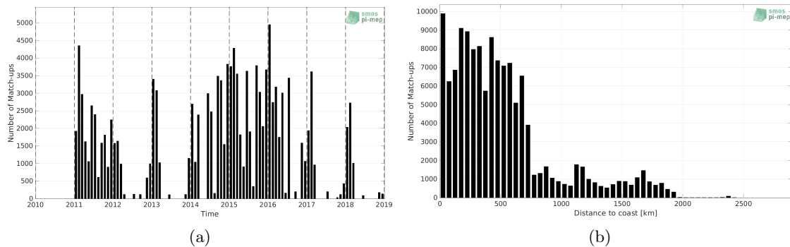
Figure 1: Number of match-ups between TSG (LEGOS-DM) and SMOS and SMAP SSS L4 OI v1 - 7 Days (LOPS) SSS as a function of time (a) and as function of the distance to coast (b) over the Indian Ocean Pi-MEP region and for the full satellite product period.
