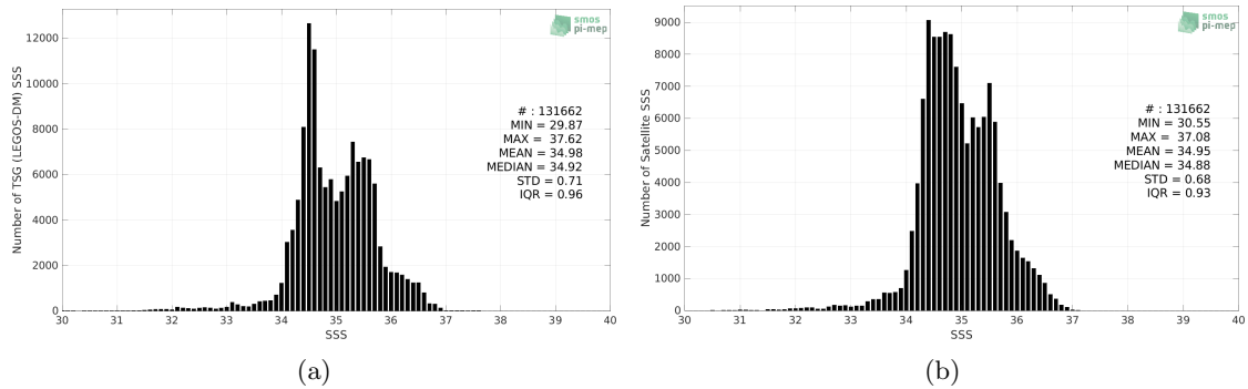
Figure 2: Histograms of SSS from TSG (LEGOS-DM) (a) and SMOS and SMAP SSS L4 OI v1 - 7 Days (LOPS) (b) considering all match-up pairs per bins of 0.1 over the Indian Ocean Pi-MEP region and for the full satellite product period.
