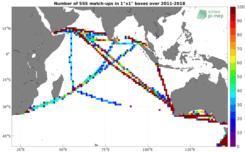
Figure 4: Number of SSS match-ups between TSG (LEGOS-DM) SSS and the SMOS and SMAP SSS L4 OI v1 - 7 Days (LOPS) SSS product for the Indian Ocean Pi-MEP region over 1^\circ \times 1^\circ boxes and for the full satellite product period.
