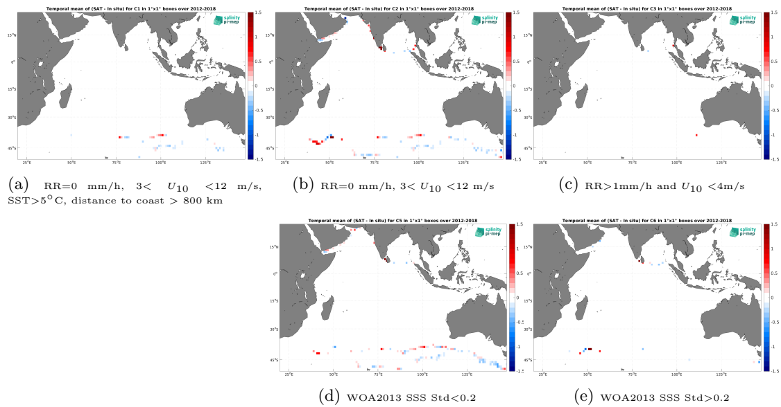
Figure 12: Temporal mean gridded over spatial boxes of size 1^\circ \times 1^\circ of \Delta\text{SSS} (SMOS and SMAP SSS L4 OI v1 - 7 Days (LOPS) - TSG (GOSUD-Sailing-ship)) for 5 different subdatasets corresponding to:RR=0 mm/h, 3 < U_{10} < 12 m/s, SST > 5^\circ\text{C} , distance to coast > 800 km (a), RR=0 mm/h, 3 < U_{10} < 12 m/s (b), RR > 1 mm/h and U_{10} < 4 m/s (c), WOA2013 SSS Std < 0.2 (d), WOA2013 SSS Std > 0.2 (e).
