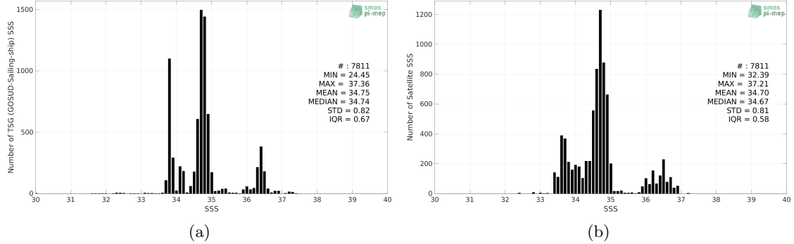
Figure 2: Histograms of SSS from TSG (GOSUD-Sailing-ship) (a) and SMOS and SMAP SSS L4 OI v1 - 7 Days (LOPS) (b) considering all match-up pairs per bins of 0.1 over the Indian Ocean Pi-MEP region and for the full satellite product period.
