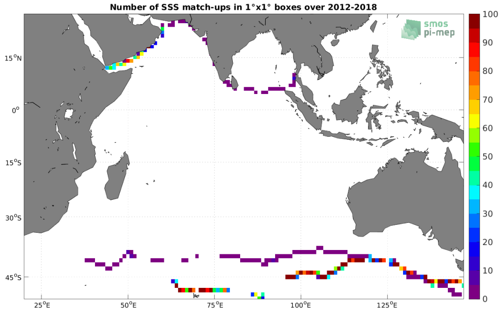
Figure 4: Number of SSS match-ups between TSG (GOSUD-Sailing-ship) SSS and the SMOS and SMAP SSS L4 OI v1 - 7 Days (LOPS) SSS product for the Indian Ocean Pi-MEP region over 1^\circ \times 1^\circ boxes and for the full satellite product period.
