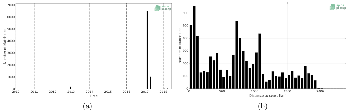
Figure 1: Number of match-ups between TSG (GOSUD-Sailing-ship) and SMOS and SMAP SSS L4 OI v1 - 7 Days (LOPS) SSS as a function of time (a) and as function of the distance to coast (b) over the Indian Ocean Pi-MEP region and for the full satellite product period.
