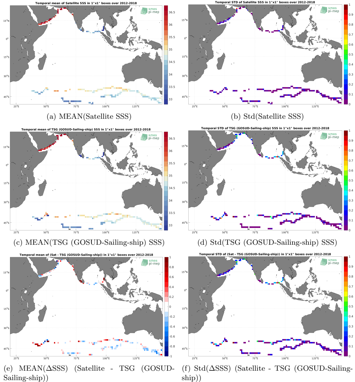
Figure 6: Temporal mean (left) and Std (right) of SSS from SMOS and SMAP SSS L4 OI v1 - 7 Days (LOPS) (top), TSG (GOSUD-Sailing-ship) (middle), and of \Delta SSS (Satellite - TSG (GOSUD-Sailing-ship)). Only match-up pairs are used to generate these maps.
