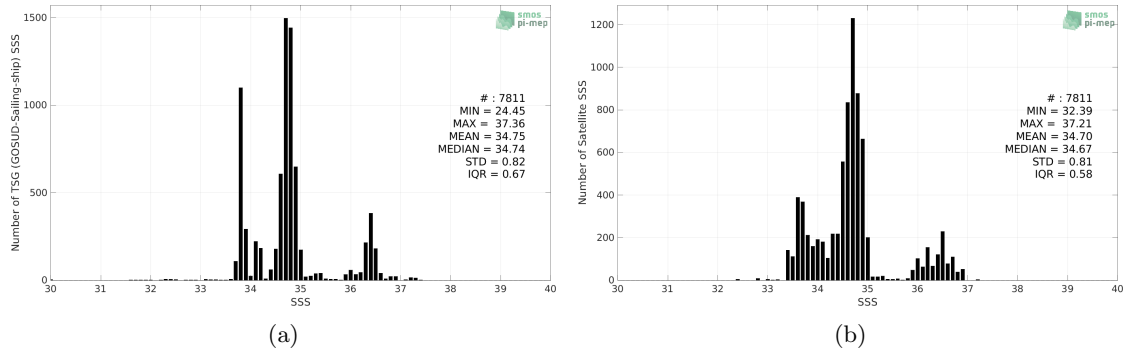
Figure 2: Histograms of SSS from TSG (GOSUD-Sailing-ship) (a) and SMOS and SMAP SSS L4 OI v1 - 7 Days (LOPS) (b) considering all match-up pairs per bins of 0.1 over the Indian Ocean Pi-MEP region and for the full satellite product period.
