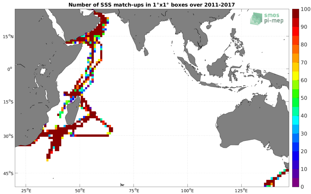
Figure 4: Number of SSS match-ups between TSG (GOSUD-Research-vessel) SSS and the SMOS and SMAP SSS L4 OI v1 - 7 Days (LOPS) SSS product for the Indian Ocean Pi-MEP region over 1^\circ \times 1^\circ boxes and for the full satellite product period.
