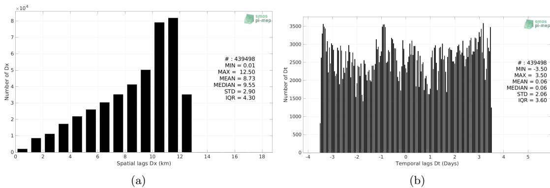
Figure 5: Histograms of the spatial (a) and temporal (b) lags between the location/time of the TSG (GOSUD-Research-vessel) measurement and the date of the corresponding SMOS and SMAP SSS L4 OI v1 - 7 Days (LOPS) SSS pixel.
