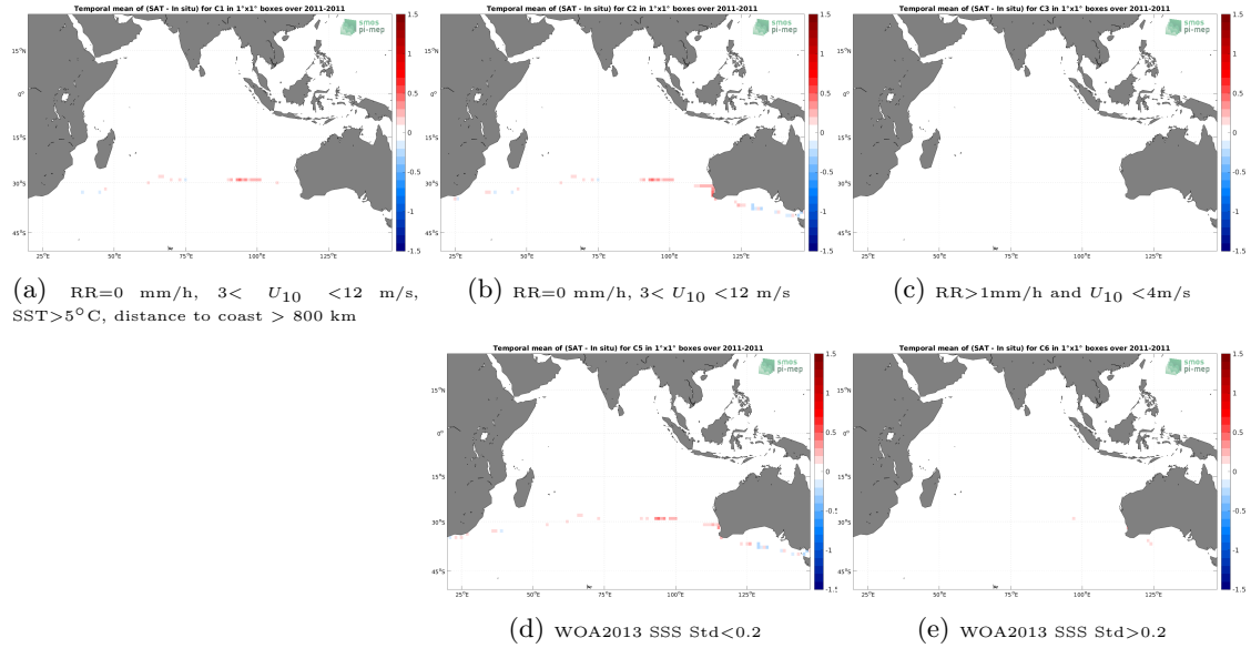
Figure 12: Temporal mean gridded over spatial boxes of size 1^{\circ}\times 1^{\circ} of \Delta\text{SSS} (SMOS and SMAP SSS L4 OI v1 - 7 Days (LOPS) - TSG (CSIC-UTM)) for 5 different subdatasets corresponding to:RR=0 mm/h, 3 < U_{10} < 12 m/s, SST >5^{\circ}\text{C} , distance to coast > 800 km (a), RR=0 mm/h, 3 < U_{10} < 12 m/s (b), RR >1 mm/h and U_{10} < 4 m/s (c), WOA2013 SSS Std <0.2 (d), WOA2013 SSS Std >0.2 (e).
