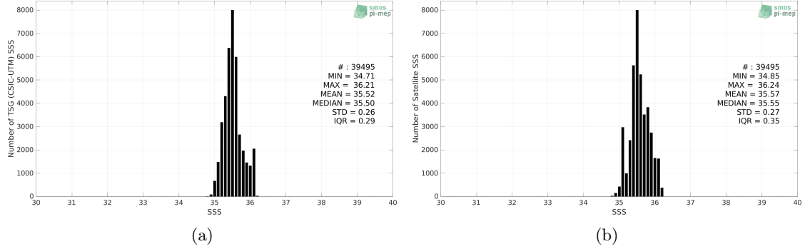
Figure 2: Histograms of SSS from TSG (CSIC-UTM) (a) and SMOS and SMAP SSS L4 OI v1 - 7 Days (LOPS) (b) considering all match-up pairs per bins of 0.1 over the Indian Ocean Pi-MEP region and for the full satellite product period.
