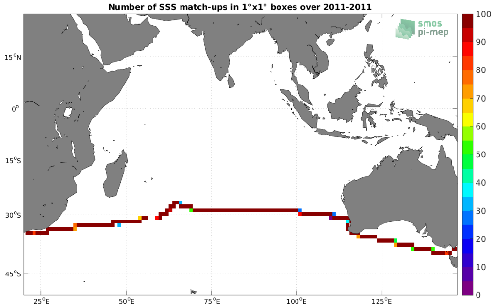
Figure 4: Number of SSS match-ups between TSG (CSIC-UTM) SSS and the SMOS and SMAP SSS L4 OI v1 - 7 Days (LOPS) SSS product for the Indian Ocean Pi-MEP region over 1^\circ \times 1^\circ boxes and for the full satellite product period.
