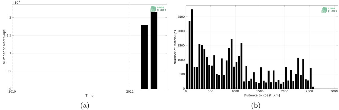
Figure 1: Number of match-ups between TSG (CSIC-UTM) and SMOS and SMAP SSS L4 OI v1 - 7 Days (LOPS) SSS as a function of time (a) and as function of the distance to coast (b) over the Indian Ocean Pi-MEP region and for the full satellite product period.
