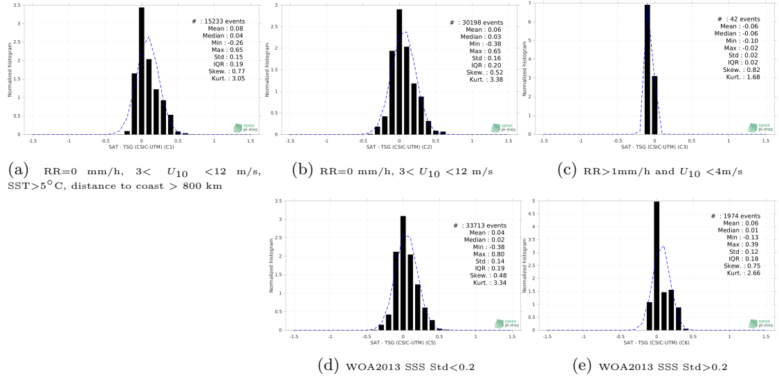
Figure 13: Normalized histogram of \Delta SSS (SMOS and SMAP SSS L4 OI v1 - 7 Days (LOPS) - TSG (CSIC-UTM)) for 5 different subdatasets corresponding to: RR=0 mm/h, 3 < U_{10} < 12 m/s, SST > 5°C, distance to coast > 800 km (a), RR=0 mm/h, 3 < U_{10} < 12 m/s (b), RR > 1mm/h and U_{10} < 4 m/s (c), WOA2013 SSS Std < 0.2 (d), WOA2013 SSS Std > 0.2 (e).
