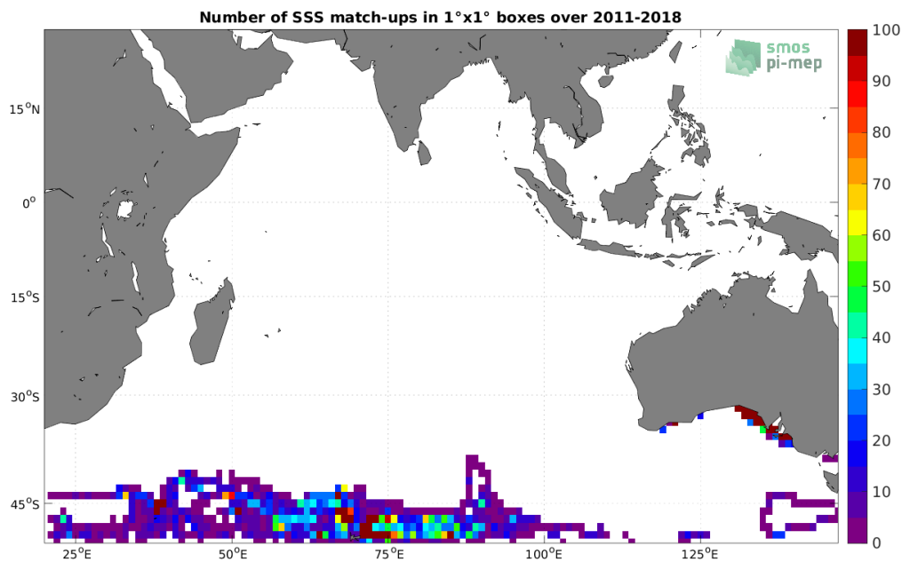
Figure 4: Number of SSS match-ups between Marine mammals SSS and the SMOS and SMAP SSS L4 OI v1 - 7 Days (LOPS) SSS product for the Indian Ocean Pi-MEP region over 1^\circ \times 1^\circ boxes and for the full satellite product period.
