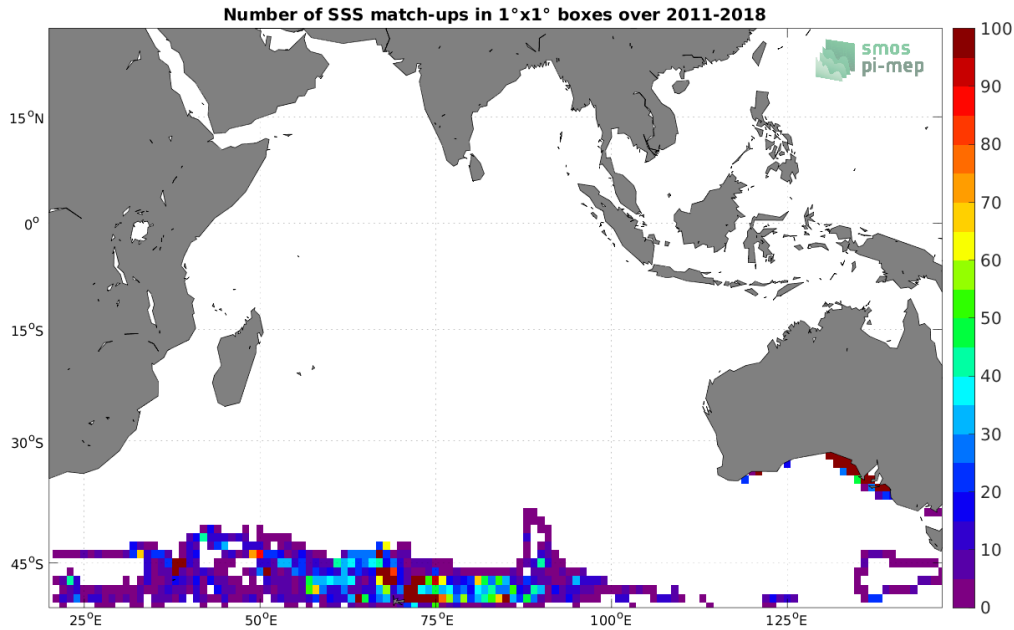
Figure 4: Number of SSS match-ups between Marine mammals SSS and the SMOS and SMAP SSS L4 OI v1 - 7 Days (LOPS) SSS product for the Indian Ocean Pi-MEP region over 1^\circ \times 1^\circ boxes and for the full satellite product period.
