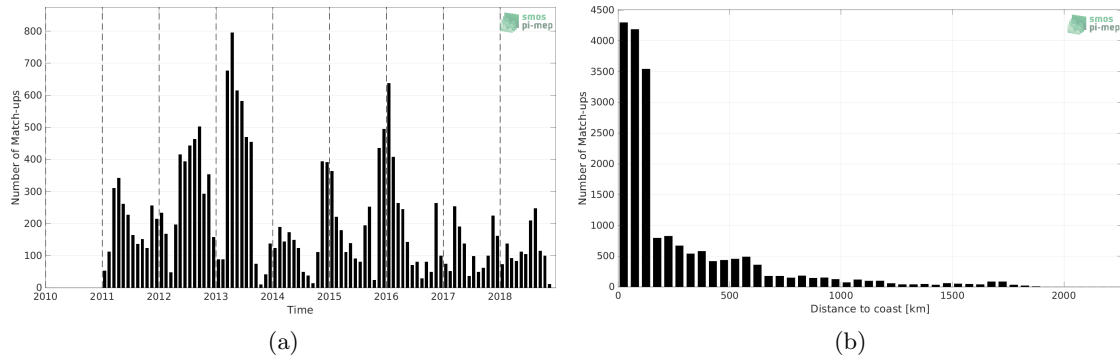
Figure 1: Number of match-ups between Marine mammals and SMOS and SMAP SSS L4 OI v1 - 7 Days (LOPS) SSS as a function of time (a) and as function of the distance to coast (b) over the Indian Ocean Pi-MEP region and for the full satellite product period.
