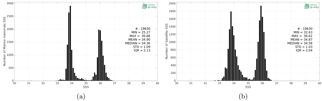
Figure 2: Histograms of SSS from Marine mammals (a) and SMOS and SMAP SSS L4 OI v1 - 7 Days (LOPS) (b) considering all match-up pairs per bins of 0.1 over the Indian Ocean Pi-MEP region and for the full satellite product period.
