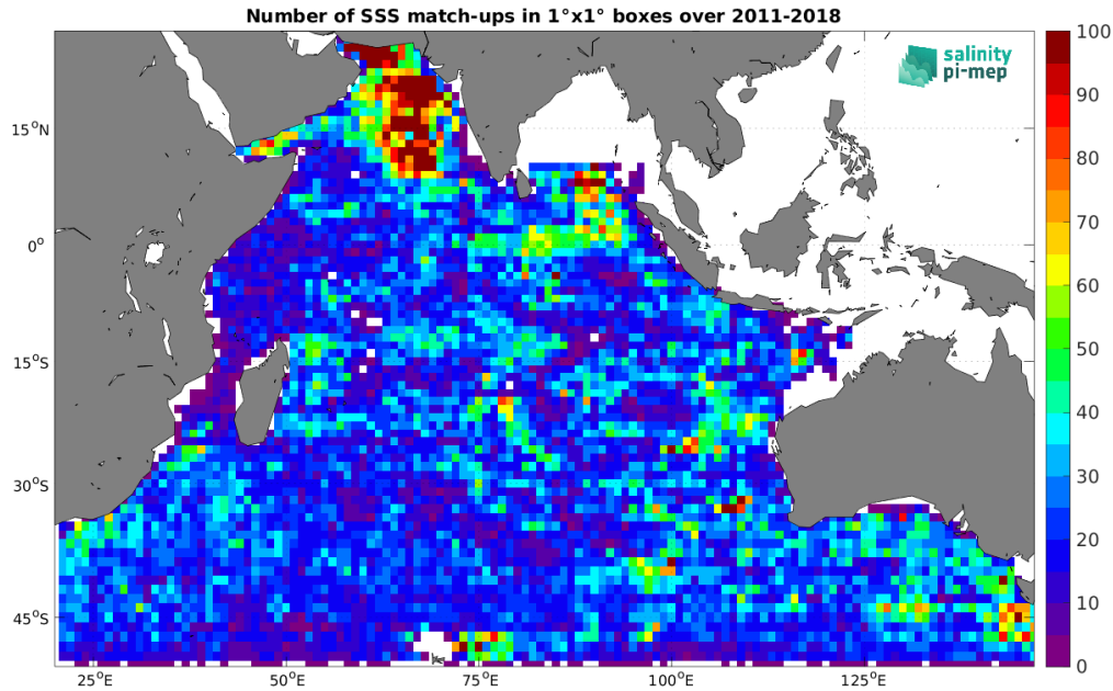
Figure 4: Number of SSS match-ups between Argo SSS and the SMOS and SMAP SSS L4 OI v1 - 7 Days (LOPS) SSS product for the Indian Ocean Pi-MEP region over 1^\circ \times 1^\circ boxes and for the full satellite product period.
