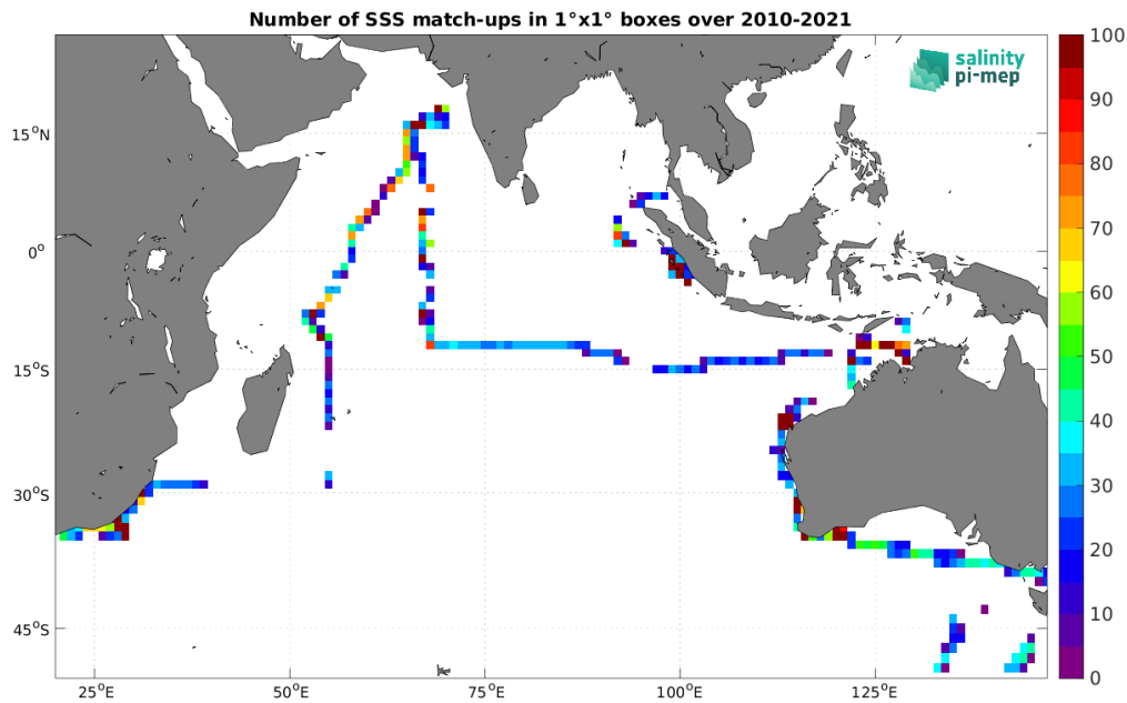
Figure 4: Number of SSS match-ups between TSG (SAMOS) SSS and the SMOS SSS L4 v1 - Weekly (CMEMS-CNR) SSS product for the Indian Ocean Pi-MEP region over 1^\circ \times 1^\circ boxes and for the full satellite product period.
