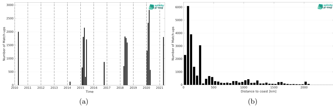
Figure 1: Number of match-ups between TSG (SAMOS) and SMOS SSS L4 v1 - Weekly (CMEMS-CNR) SSS as a function of time (a) and as function of the distance to coast (b) over the Indian Ocean Pi-MEP region and for the full satellite product period.
