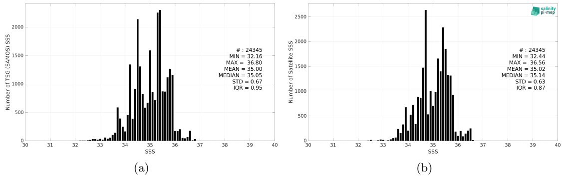
Figure 2: Histograms of SSS from TSG (SAMOS) (a) and SMOS SSS L4 v1 - Weekly (CMEMS-CNR) (b) considering all match-up pairs per bins of 0.1 over the Indian Ocean Pi-MEP region and for the full satellite product period.
