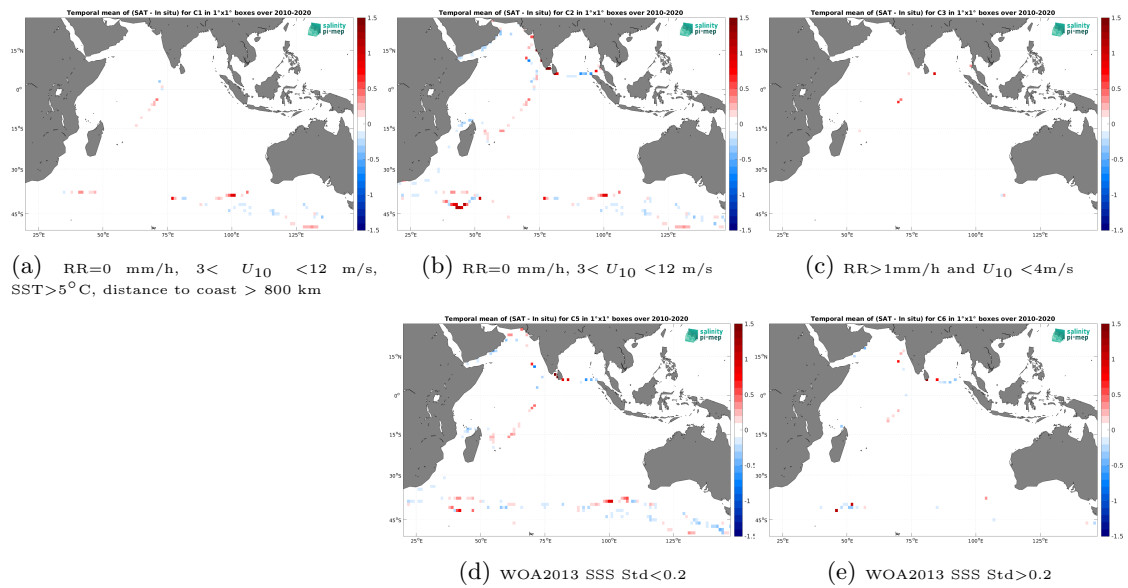
Figure 12: Temporal mean gridded over spatial boxes of size 1^\circ \times 1^\circ of \Delta\text{SSS} (SMOS SSS L4 v1 - Weekly (CMEMS-CNR) - TSG (GOSUD-Sailing-ship)) for 5 different subdatasets corresponding to: RR=0 mm/h, 3 < U_{10} < 12 m/s, SST > 5^\circ\text{C} , distance to coast > 800 km (a), RR=0 mm/h, 3 < U_{10} < 12 m/s (b), RR > 1\text{mm/h} and U_{10} < 4\text{m/s} (c), WOA2013 SSS Std < 0.2 (d), WOA2013 SSS Std > 0.2 (e).
