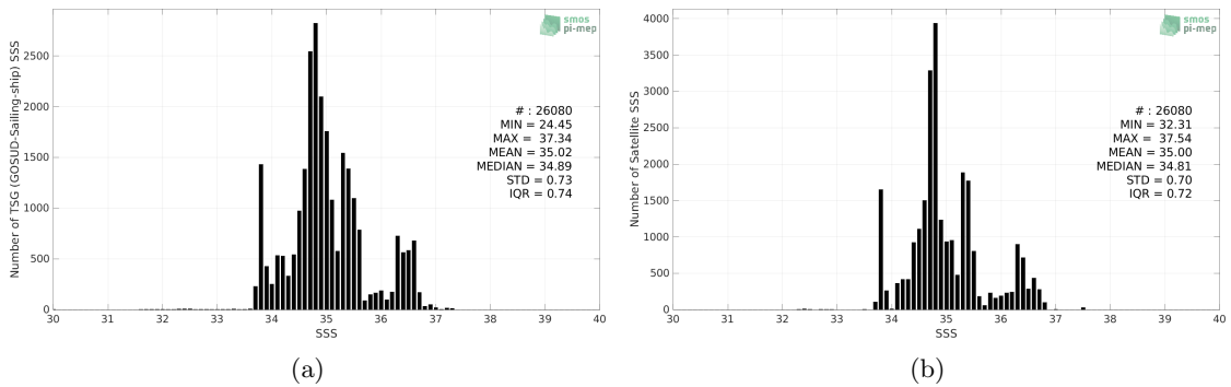
Figure 2: Histograms of SSS from TSG (GOSUD-Sailing-ship) (a) and SMOS SSS L4 v1 - Weekly (CMEMS-CNR) (b) considering all match-up pairs per bins of 0.1 over the Indian Ocean Pi-MEP region and for the full satellite product period.
