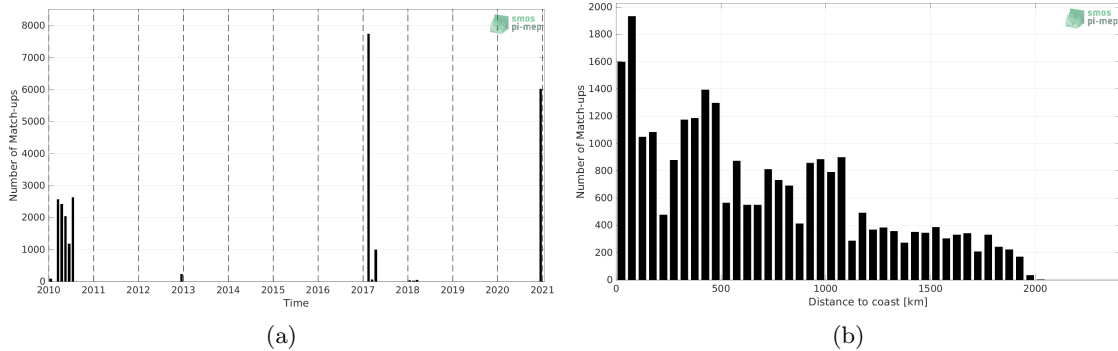
Figure 1: Number of match-ups between TSG (GOSUD-Sailing-ship) and SMOS SSS L4 v1 - Weekly (CMEMS-CNR) SSS as a function of time (a) and as function of the distance to coast (b) over the Indian Ocean Pi-MEP region and for the full satellite product period.
