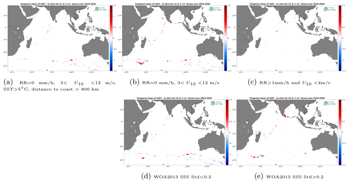
Figure 12: Temporal mean gridded over spatial boxes of size 1^\circ \times 1^\circ of \Delta SSS (SMOS SSS L4 v1 - Weekly (CMEMS-CNR) - TSG (GOSUD-Sailing-ship)) for 5 different subdatasets corresponding to: RR=0 mm/h, 3 < U_{10} < 12 m/s, SST > 5^\circ\text{C} , distance to coast > 800 km (a), RR=0 mm/h, 3 < U_{10} < 12 m/s (b), RR > 1\text{mm/h} and U_{10} < 4\text{m/s} (c), WOA2013 SSS Std < 0.2 (d), WOA2013 SSS Std > 0.2 (e).
