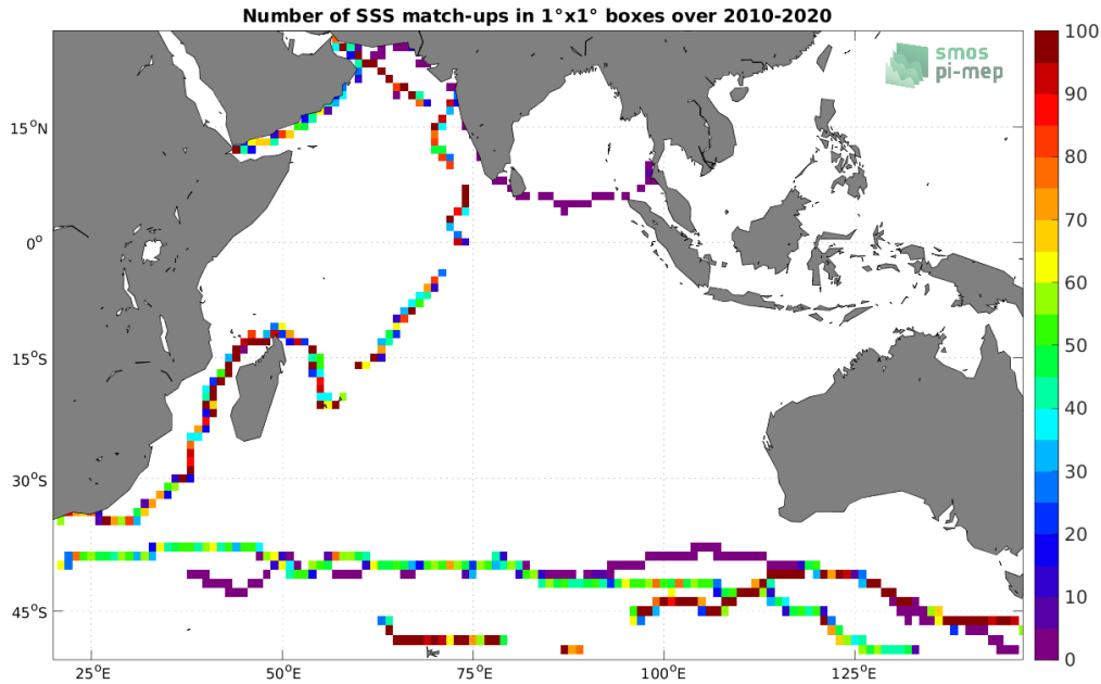
Figure 4: Number of SSS match-ups between TSG (GOSUD-Sailing-ship) SSS and the SMOS SSS L4 v1 - Weekly (CMEMS-CNR) SSS product for the Indian Ocean Pi-MEP region over 1^\circ \times 1^\circ boxes and for the full satellite product period.
