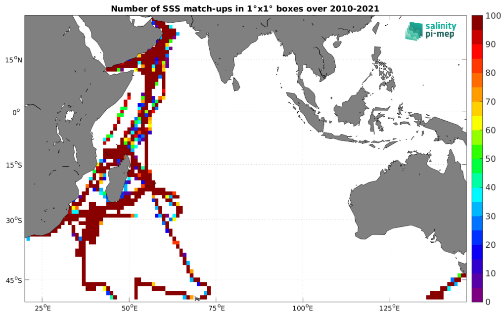
Figure 4: Number of SSS match-ups between TSG (GOSUD-Research-vessel) SSS and the SMOS SSS L4 v1 - Weekly (CMEMS-CNR) SSS product for the Indian Ocean Pi-MEP region over 1^\circ \times 1^\circ boxes and for the full satellite product period.
