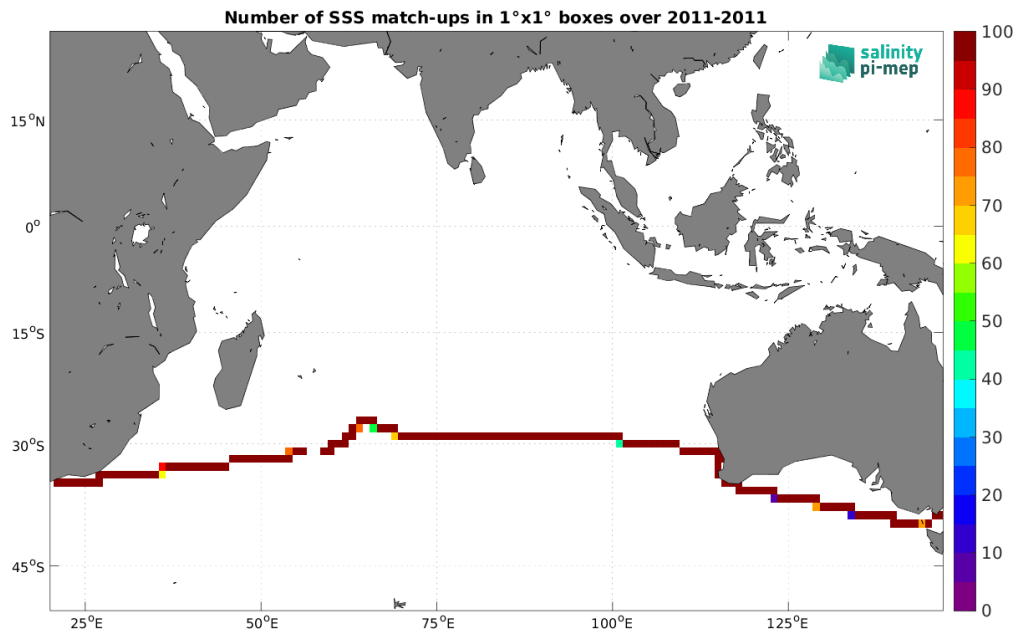
Figure 4: Number of SSS match-ups between TSG (CSIC-UTM) SSS and the SMOS SSS L4 v1 - Weekly (CMEMS-CNR) SSS product for the Indian Ocean Pi-MEP region over 1^{\circ} \times 1^{\circ} boxes and for the full satellite product period.
