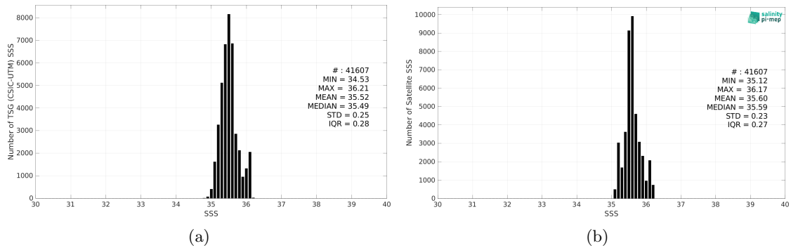
Figure 2: Histograms of SSS from TSG (CSIC-UTM) (a) and SMOS SSS L4 v1 - Weekly (CMEMS-CNR) (b) considering all match-up pairs per bins of 0.1 over the Indian Ocean Pi-MEP region and for the full satellite product period.
