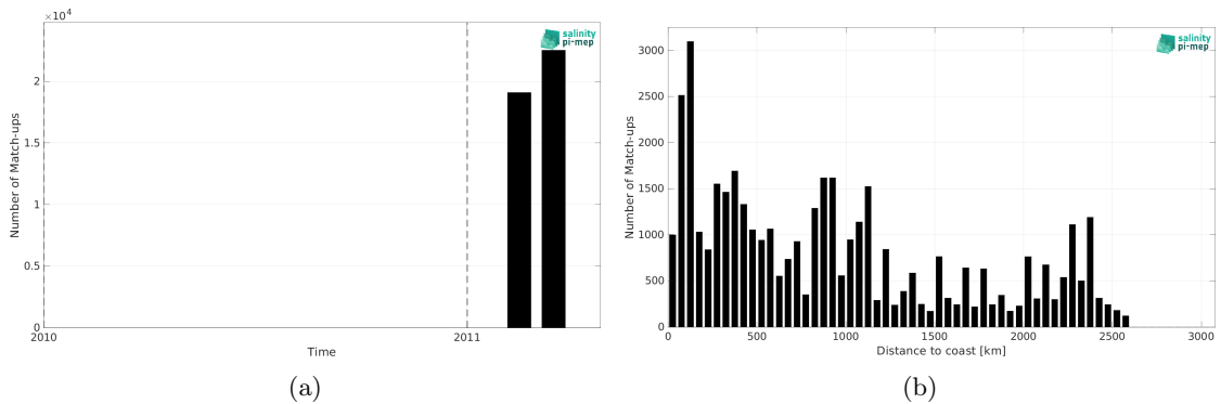
Figure 1: Number of match-ups between TSG (CSIC-UTM) and SMOS SSS L4 v1 - Weekly (CMEMS-CNR) SSS as a function of time (a) and as function of the distance to coast (b) over the Indian Ocean Pi-MEP region and for the full satellite product period.
