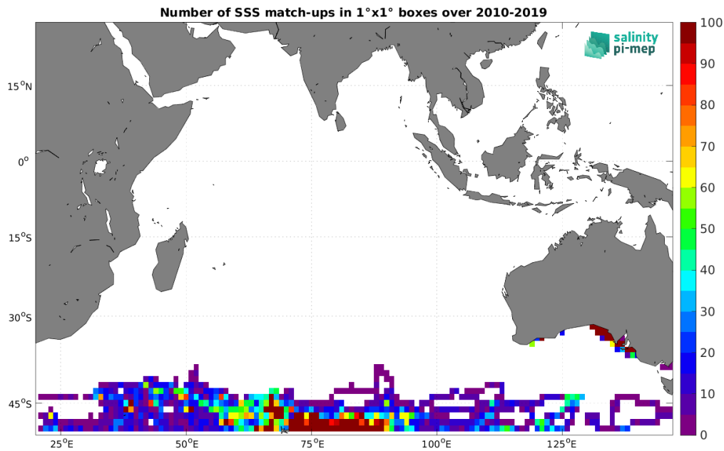
Figure 4: Number of SSS match-ups between Marine mammals SSS and the SMOS SSS L4 v1 - Weekly (CMEMS-CNR) SSS product for the Indian Ocean Pi-MEP region over 1^\circ \times 1^\circ boxes and for the full satellite product period.
