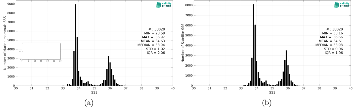
Figure 2: Histograms of SSS from Marine mammals (a) and SMOS SSS L4 v1 - Weekly (CMEMS-CNR) (b) considering all match-up pairs per bins of 0.1 over the Indian Ocean Pi-MEP region and for the full satellite product period.
