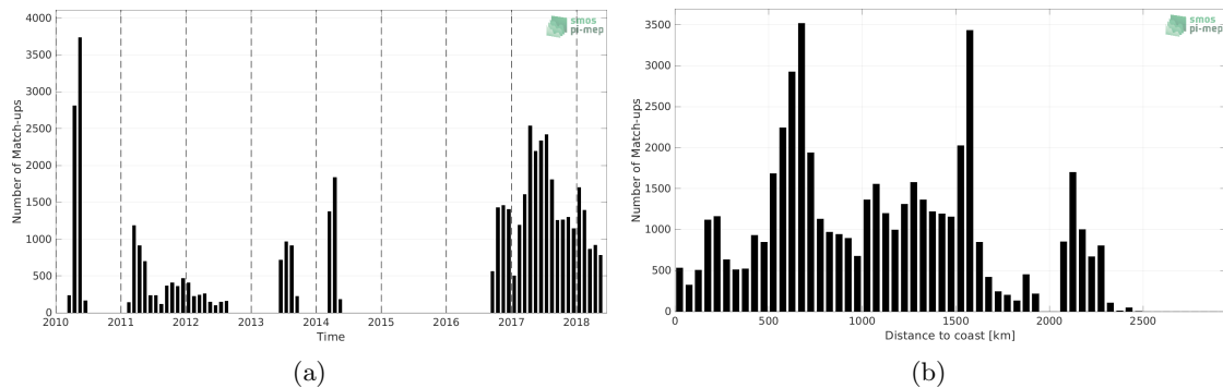
Figure 1: Number of match-ups between Surface drifters and SMOS SSS L4 v1 - Weekly (CMEMS-CNR) SSS as a function of time (a) and as function of the distance to coast (b) over the Indian Ocean Pi-MEP region and for the full satellite product period.
