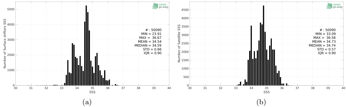
Figure 2: Histograms of SSS from Surface drifters (a) and SMOS SSS L4 v1 - Weekly (CMEMS-CNR) (b) considering all match-up pairs per bins of 0.1 over the Indian Ocean Pi-MEP region and for the full satellite product period.
