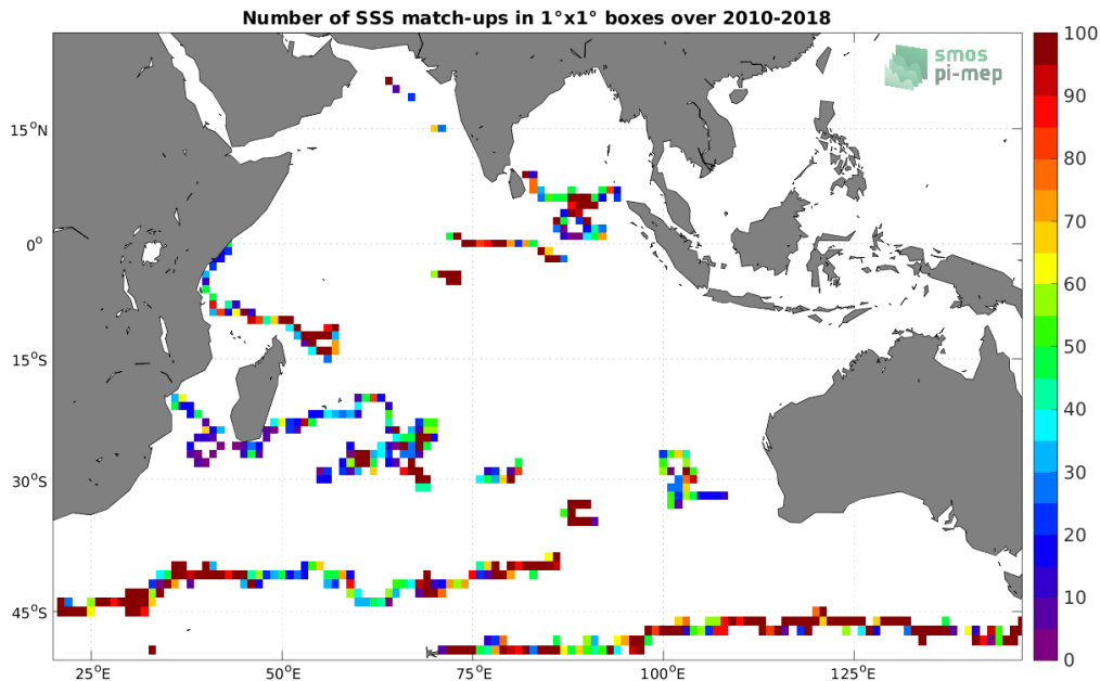
Figure 3: Number of SSS match-ups between Surface drifters SSS and the SMOS SSS L4 v1 - Weekly (CMEMS-CNR) SSS product for the Indian Ocean Pi-MEP region over 1^\circ \times 1^\circ boxes and for the full satellite product period.
