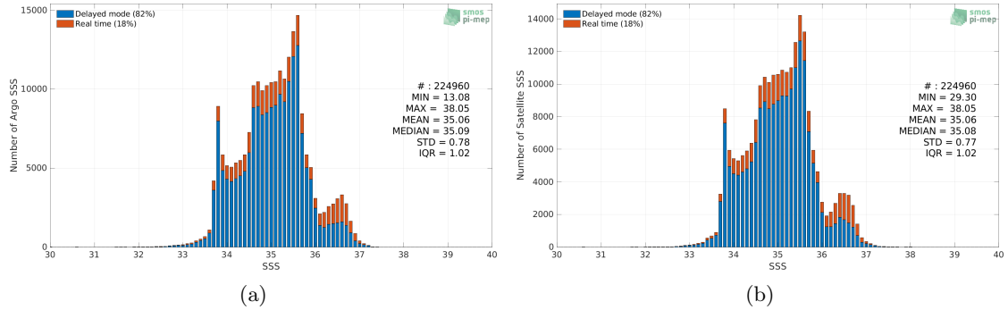
Figure 2: Histograms of SSS from Argo (a) and SMOS SSS L4 v1 - Weekly (CMEMS-CNR) (b) considering all match-up pairs per bins of 0.1 over the Indian Ocean Pi-MEP region and for the full satellite product period.
