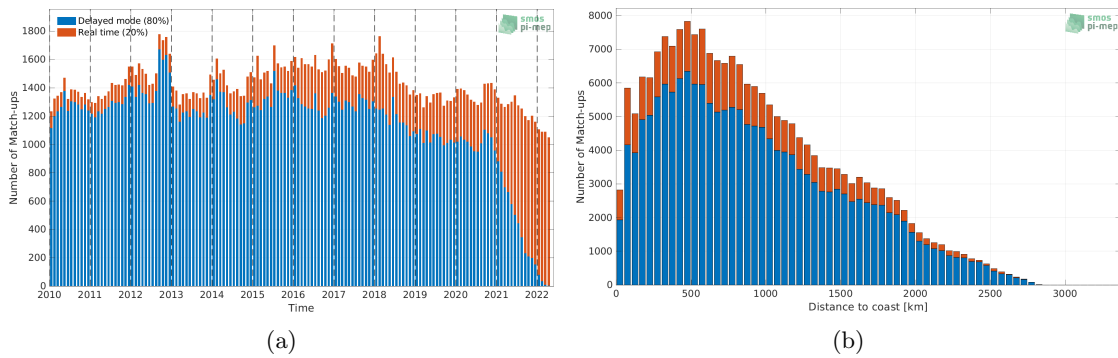
Figure 1: Number of match-ups between Argo and SMOS SSS L4 v1 - Weekly (CMEMS-CNR) SSS as a function of time (a) and as function of the distance to coast (b) over the Indian Ocean Pi-MEP region and for the full satellite product period.
