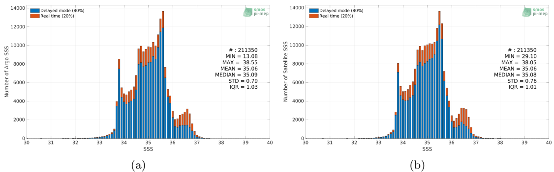
Figure 2: Histograms of SSS from Argo (a) and SMOS SSS L4 v1 - Weekly (CMEMS-CNR) (b) considering all match-up pairs per bins of 0.1 over the Indian Ocean Pi-MEP region and for the full satellite product period.
