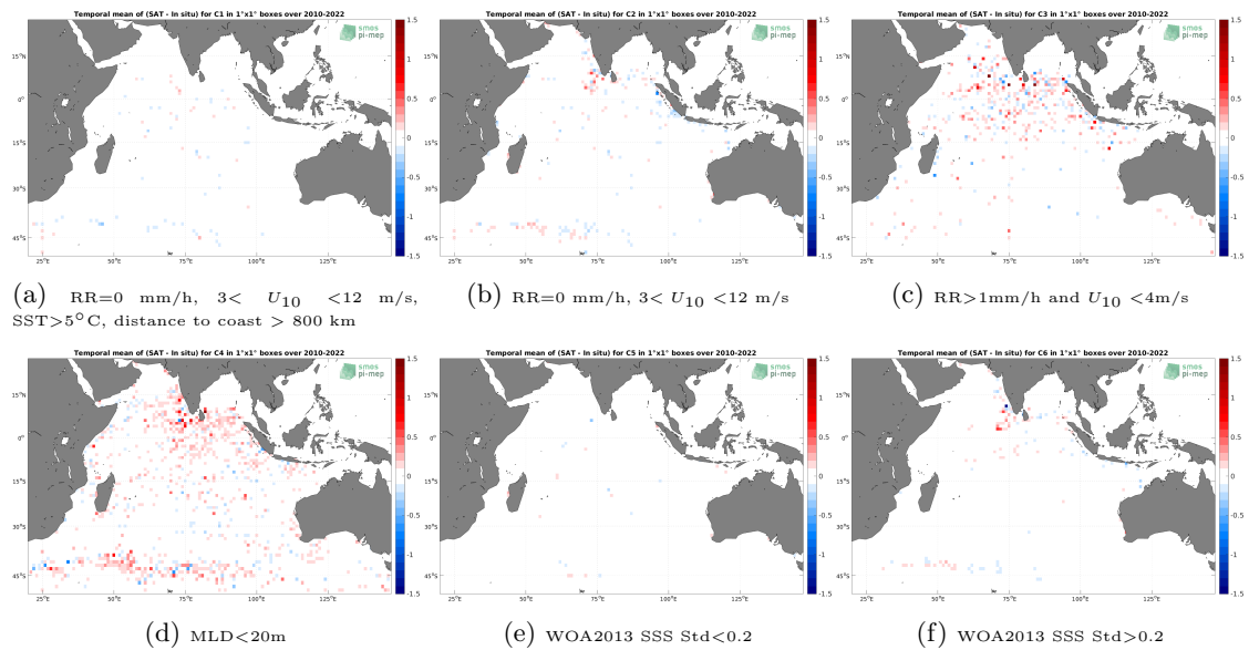
Figure 12: Temporal mean gridded over spatial boxes of size 1^\circ \times 1^\circ of \Delta SSS (SMOS SSS L4 v1 - Weekly (CMEMS-CNR) - Argo) for 6 different subdatasets corresponding to:RR=0 mm/h, 3 < U_{10} < 12 m/s, SST >5^\circ C, distance to coast > 800 km (a), RR=0 mm/h, 3 < U_{10} < 12 m/s (b), RR >1 mm/h and U_{10} < 4 m/s (c),MLD <20 m (d),WOA2013 SSS Std <0.2 (e),WOA2013 SSS Std >0.2 (f).
