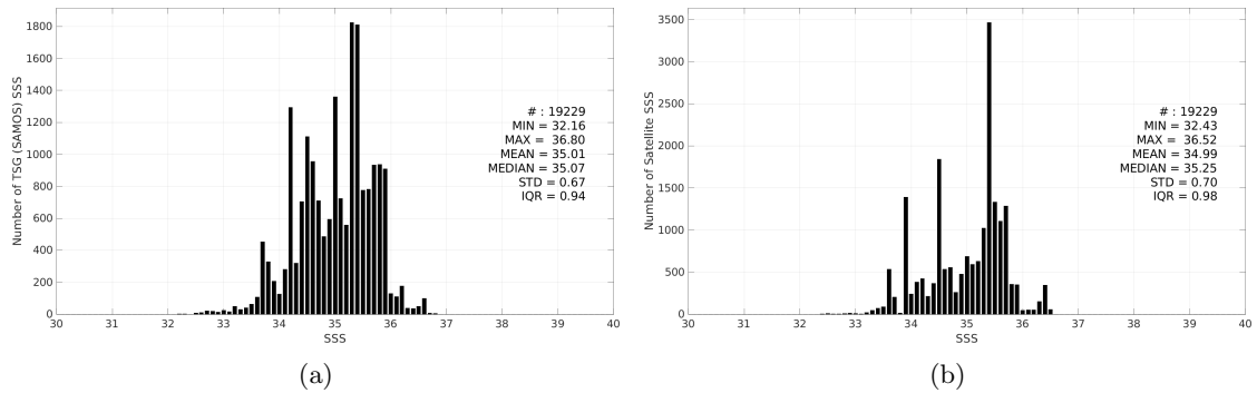
Figure 3: Histograms of SSS from TSG (SAMOS) (a) and SMOS SSS L4 v1 - Monthly (CMEMS-CNR) (b) considering all match-up pairs per bins of 0.1 over the Indian Ocean Pi-MEP region and for the full satellite product period.
