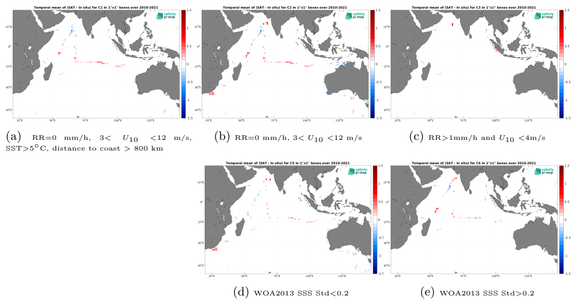
Figure 14: Temporal mean gridded over spatial boxes of size 1^\circ \times 1^\circ of \Delta SSS (SMOS SSS L4 v1 - Monthly (CMEMS-CNR) - TSG (SAMOS)) for 5 different subdatasets corresponding to:RR=0 mm/h, 3 < U_{10} < 12 m/s, SST > 5^\circ\text{C} , distance to coast > 800 km (a), RR=0 mm/h, 3 < U_{10} < 12 m/s (b), RR > 1 mm/h and U_{10} < 4 m/s (c), WOA2013 SSS Std < 0.2 (d), WOA2013 SSS Std > 0.2 (e).
