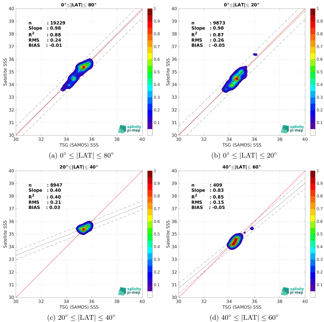
Figure 10: Contour maps of the concentration of SMOS SSS L4 v1 - Monthly (CMEMS-CNR) SSS (y-axis) versus TSG (SAMOS) SSS (x-axis) at match-up pairs for different latitude bands. For each plot, the red line shows x=y . The black thin and dashed lines indicate a linear fit through the data cloud and the \pm 95\% confidence levels, respectively. The number match-up pairs n , the slope and R^2 coefficient of the linear fit, the root mean square (RMS) and the mean bias between satellite and in situ data are indicated for each latitude band in each plots.
