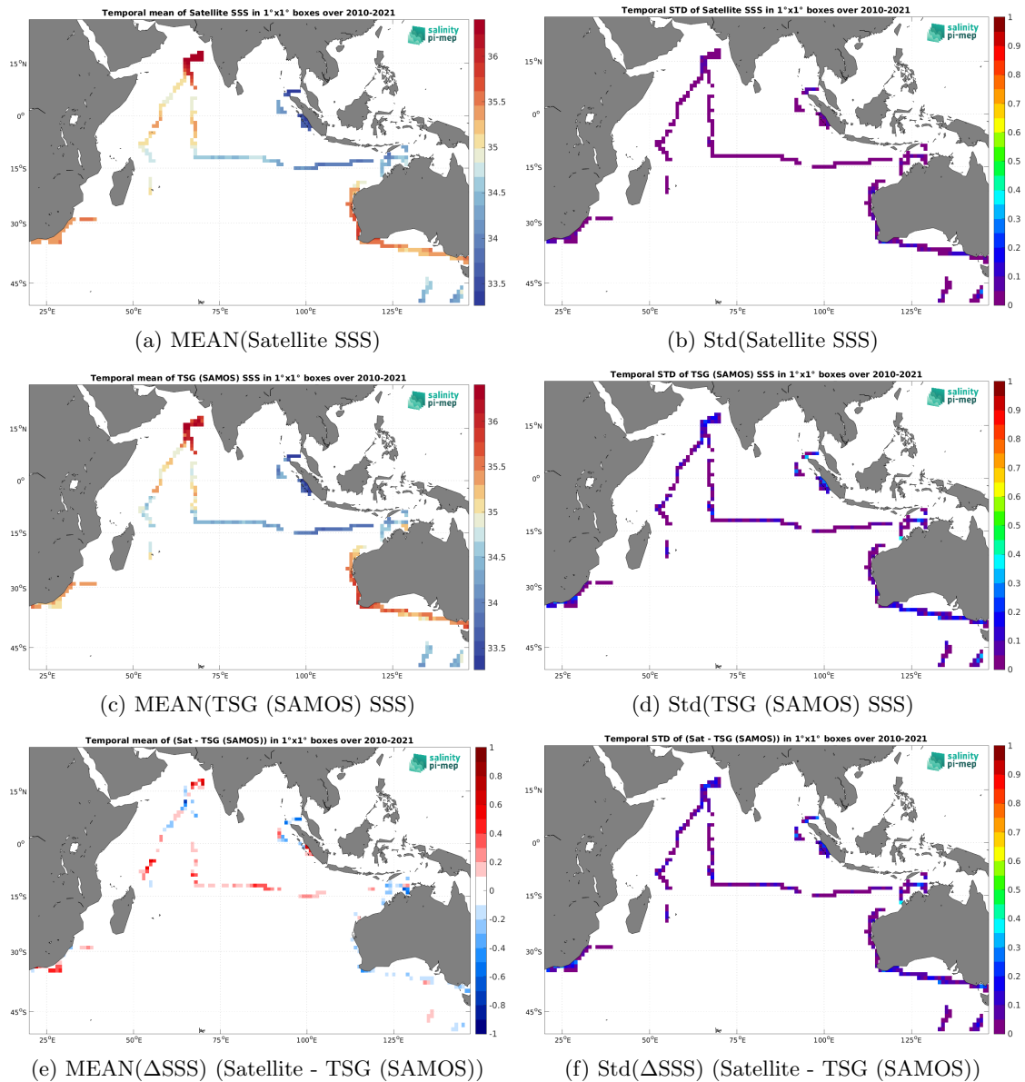
Figure 7: Temporal mean (left) and Std (right) of SSS from SMOS SSS L4 v1 - Monthly (CMEMS-CNR) (top), TSG (SAMOS) (middle), and of \Delta SSS (Satellite - TSG (SAMOS)). Only match-up pairs are used to generate these maps.
