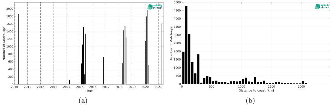
Figure 2: Number of match-ups between TSG (SAMOS) and SMOS SSS L4 v1 - Monthly (CMEMS-CNR) SSS as a function of time (a) and as function of the distance to coast (b) over the Indian Ocean Pi-MEP region and for the full satellite product period.
