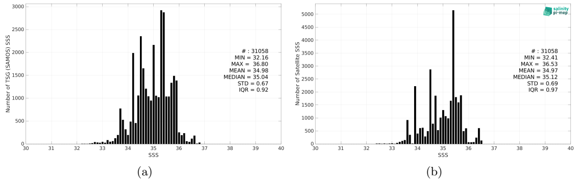
Figure 2: Histograms of SSS from TSG (SAMOS) (a) and SMOS SSS L4 v1 - Monthly (CMEMS-CNR) (b) considering all match-up pairs per bins of 0.1 over the Indian Ocean Pi-MEP region and for the full satellite product period.
