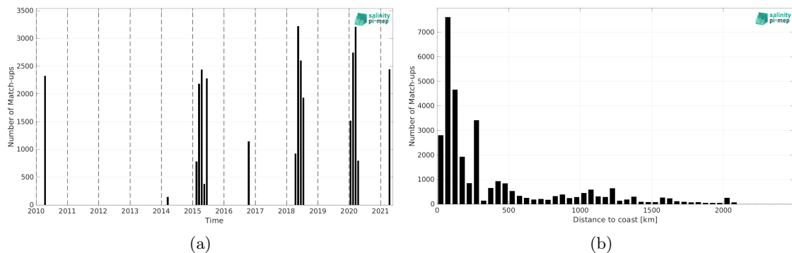
Figure 1: Number of match-ups between TSG (SAMOS) and SMOS SSS L4 v1 - Monthly (CMEMS-CNR) SSS as a function of time (a) and as function of the distance to coast (b) over the Indian Ocean Pi-MEP region and for the full satellite product period.
