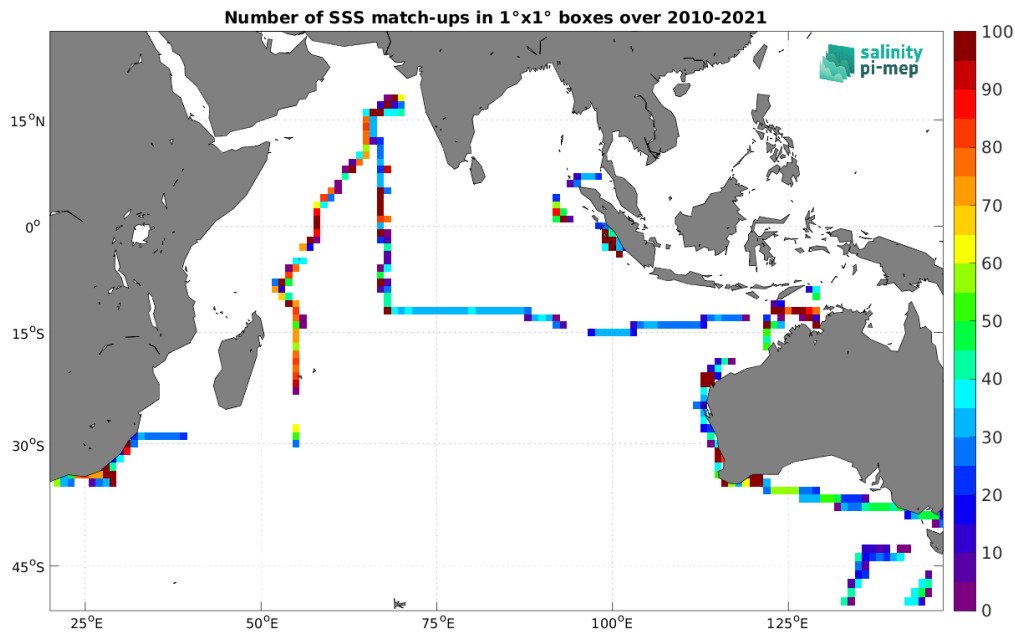
Figure 4: Number of SSS match-ups between TSG (SAMOS) SSS and the SMOS SSS L4 v1 - Monthly (CMEMS-CNR) SSS product for the Indian Ocean Pi-MEP region over 1^\circ \times 1^\circ boxes and for the full satellite product period.
