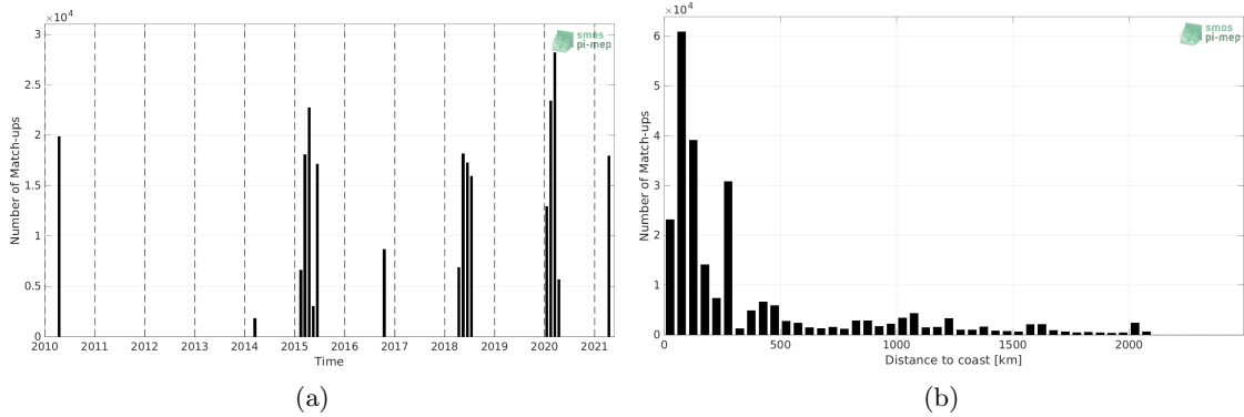
Figure 1: Number of match-ups between TSG (SAMOS) and SMOS SSS L4 v1 - Monthly (CMEMS-CNR) SSS as a function of time (a) and as function of the distance to coast (b) over the Indian Ocean Pi-MEP region and for the full satellite product period.
