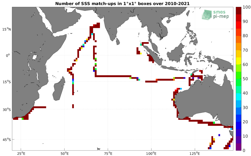
Figure 4: Number of SSS match-ups between TSG (SAMOS) SSS and the SMOS SSS L4 v1 - Monthly (CMEMS-CNR) SSS product for the Indian Ocean Pi-MEP region over 1^{\circ} \times 1^{\circ} boxes and for the full satellite product period.
