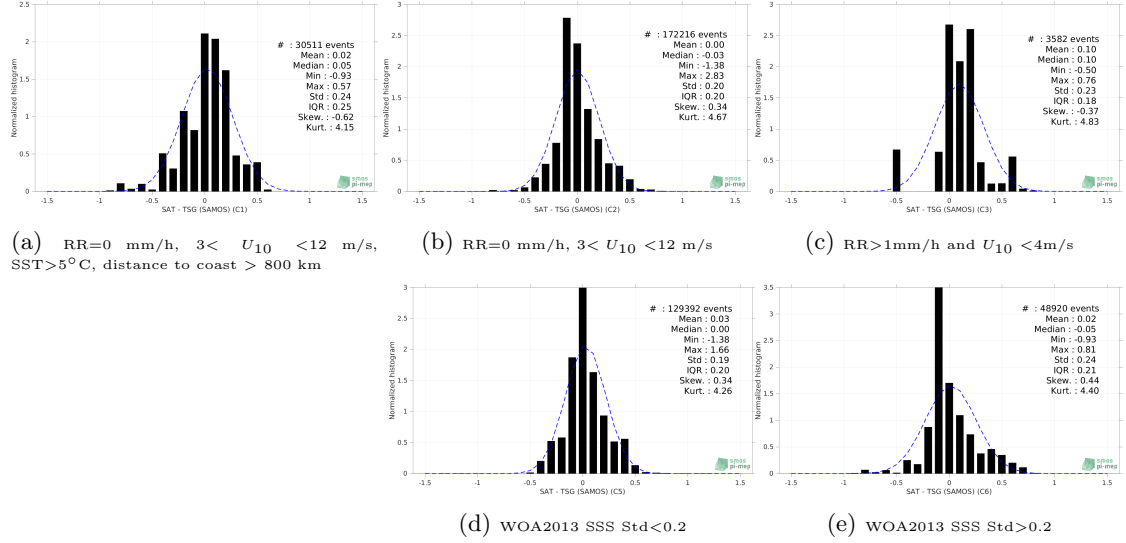
Figure 13: Normalized histogram of \Delta SSS (SMOS SSS L4 v1 - Monthly (CMEMS-CNR) - TSG (SAMOS)) for 5 different subdatasets corresponding to: RR=0 mm/h, 3 < U_{10} < 12 m/s, SST > 5°C, distance to coast > 800 km (a), RR=0 mm/h, 3 < U_{10} < 12 m/s (b), RR > 1mm/h and U_{10} < 4 m/s (c), WOA2013 SSS Std < 0.2 (d), WOA2013 SSS Std > 0.2 (e).
