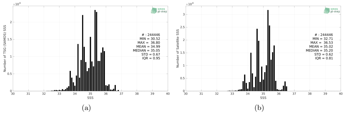
Figure 2: Histograms of SSS from TSG (SAMOS) (a) and SMOS SSS L4 v1 - Monthly (CMEMS-CNR) (b) considering all match-up pairs per bins of 0.1 over the Indian Ocean Pi-MEP region and for the full satellite product period.
