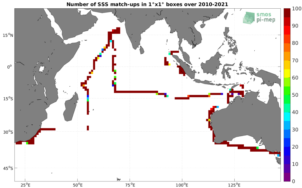
Figure 4: Number of SSS match-ups between TSG (SAMOS) SSS and the SMOS SSS L4 v1 - Monthly (CMEMS-CNR) SSS product for the Indian Ocean Pi-MEP region over 1^\circ \times 1^\circ boxes and for the full satellite product period.
