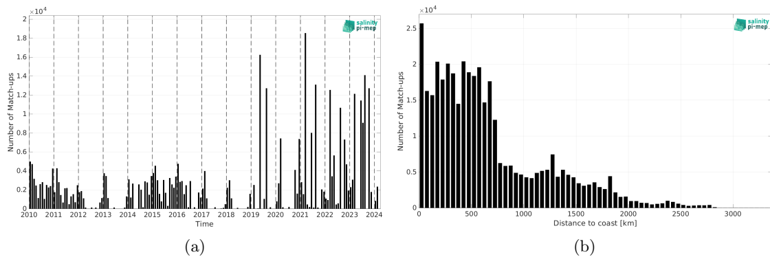
Figure 2: Number of match-ups between TSG (LEGOS-DM) and SMOS SSS L4 v1 - Monthly (CMEMS-CNR) SSS as a function of time (a) and as function of the distance to coast (b) over the Indian Ocean Pi-MEP region and for the full satellite product period.
