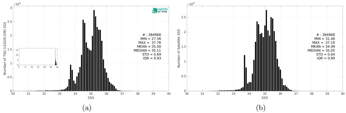
Figure 3: Histograms of SSS from TSG (LEGOS-DM) (a) and SMOS SSS L4 v1 - Monthly (CMEMS-CNR) (b) considering all match-up pairs per bins of 0.1 over the Indian Ocean Pi-MEP region and for the full satellite product period.
