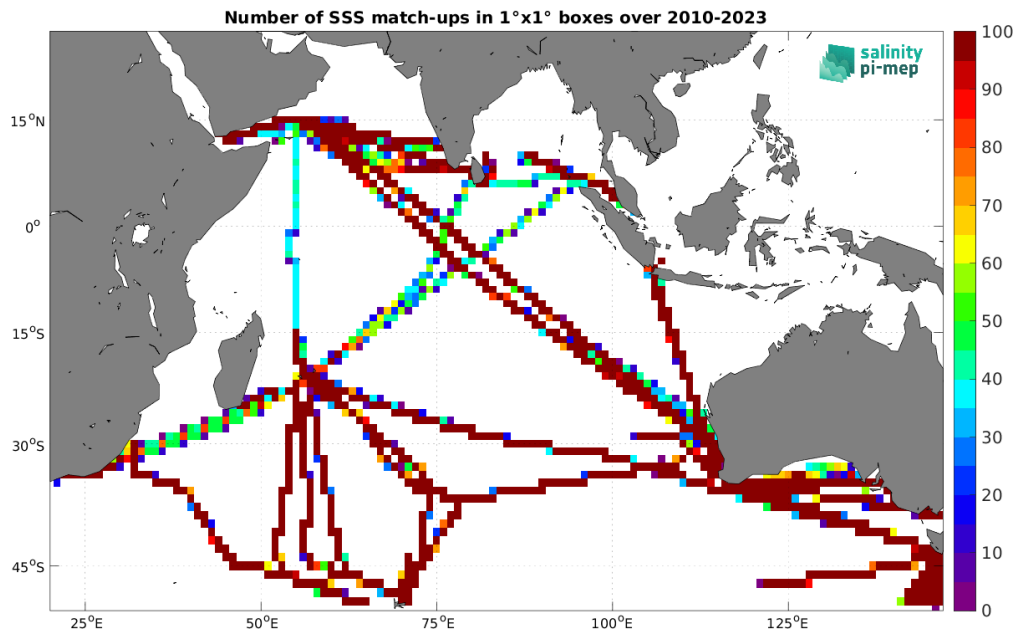
Figure 4: Number of SSS match-ups between TSG (LEGOS-DM) SSS and the SMOS SSS L4 v1 - Monthly (CMEMS-CNR) SSS product for the Indian Ocean Pi-MEP region over 1^\circ \times 1^\circ boxes and for the full satellite product period.
