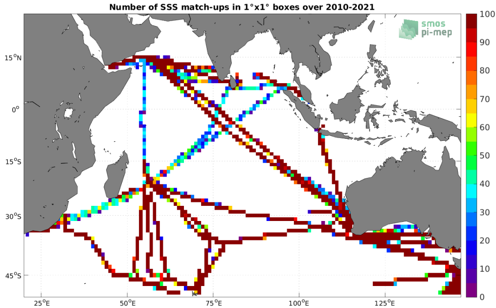
Figure 4: Number of SSS match-ups between TSG (LEGOS-DM) SSS and the SMOS SSS L4 v1 - Monthly (CMEMS-CNR) SSS product for the Indian Ocean Pi-MEP region over 1^\circ \times 1^\circ boxes and for the full satellite product period.
