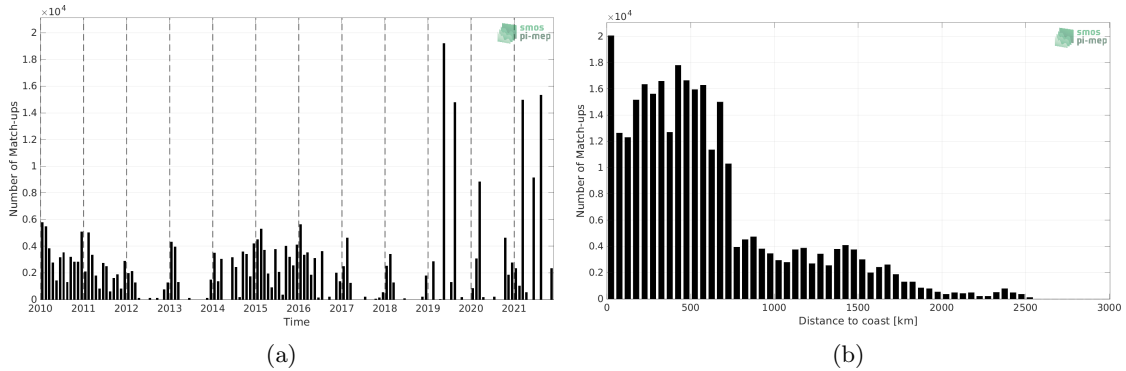
Figure 1: Number of match-ups between TSG (LEGOS-DM) and SMOS SSS L4 v1 - Monthly (CMEMS-CNR) SSS as a function of time (a) and as function of the distance to coast (b) over the Indian Ocean Pi-MEP region and for the full satellite product period.
