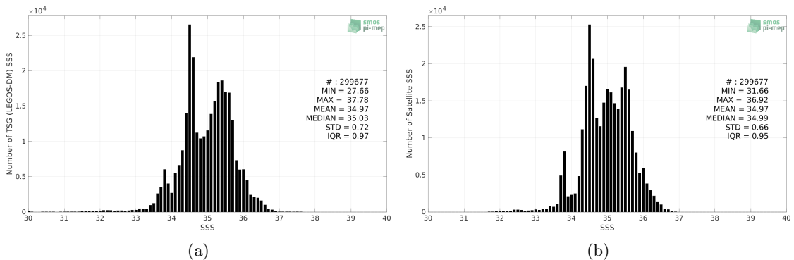
Figure 2: Histograms of SSS from TSG (LEGOS-DM) (a) and SMOS SSS L4 v1 - Monthly (CMEMS-CNR) (b) considering all match-up pairs per bins of 0.1 over the Indian Ocean Pi-MEP region and for the full satellite product period.
