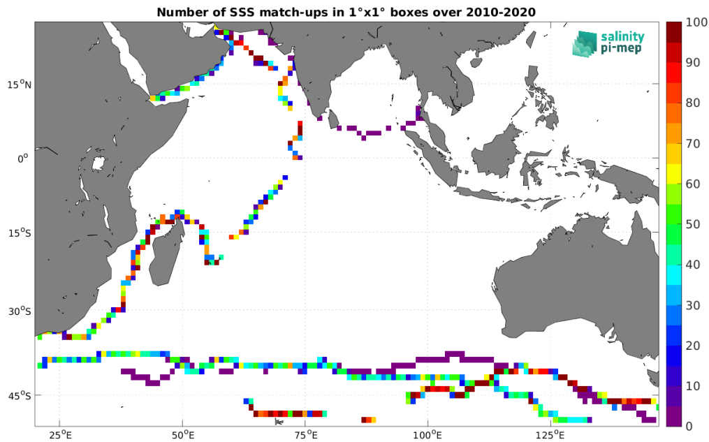
Figure 5: Number of SSS match-ups between TSG (GOSUD-Sailing-ship) SSS and the SMOS SSS L4 v1 - Monthly (CMEMS-CNR) SSS product for the Indian Ocean Pi-MEP region over 1^\circ \times 1^\circ boxes and for the full satellite product period.
