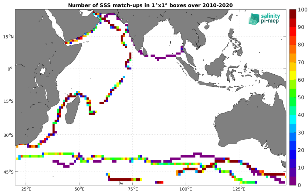
Figure 4: Number of SSS match-ups between TSG (GOSUD-Sailing-ship) SSS and the SMOS SSS L4 v1 - Monthly (CMEMS-CNR) SSS product for the Indian Ocean Pi-MEP region over 1^\circ \times 1^\circ boxes and for the full satellite product period.
