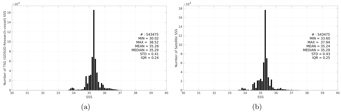
Figure 3: Histograms of SSS from TSG (GOSUD-Research-vessel) (a) and SMOS SSS L4 v1 - Monthly (CMEMS-CNR) (b) considering all match-up pairs per bins of 0.1 over the Indian Ocean Pi-MEP region and for the full satellite product period.
