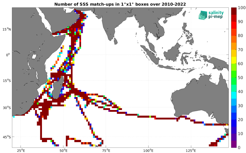
Figure 5: Number of SSS match-ups between TSG (GOSUD-Research-vessel) SSS and the SMOS SSS L4 v1 - Monthly (CMEMS-CNR) SSS product for the Indian Ocean Pi-MEP region over 1^\circ \times 1^\circ boxes and for the full satellite product period.
