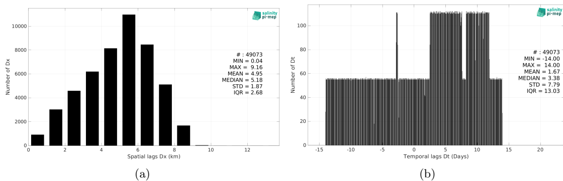
Figure 5: Histograms of the spatial (a) and temporal (b) lags between the location/time of the TSG (CSIC-UTM) measurement and the date of the corresponding SMOS SSS L4 v1 - Monthly (CMEMS-CNR) SSS pixel.
