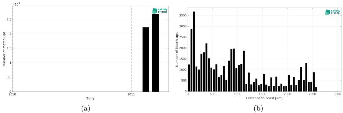
Figure 1: Number of match-ups between TSG (CSIC-UTM) and SMOS SSS L4 v1 - Monthly (CMEMS-CNR) SSS as a function of time (a) and as function of the distance to coast (b) over the Indian Ocean Pi-MEP region and for the full satellite product period.
