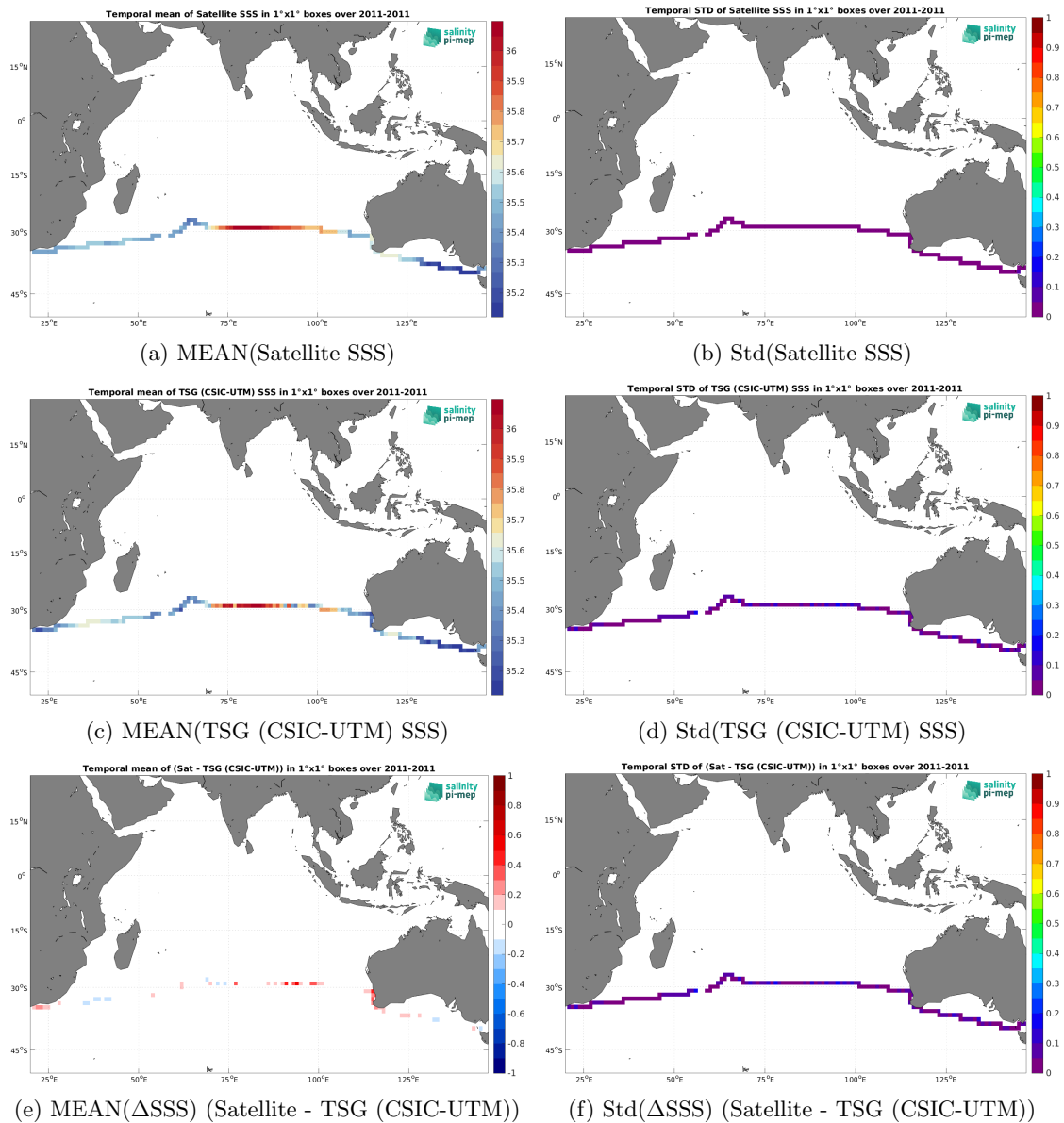
Figure 6: Temporal mean (left) and Std (right) of SSS from SMOS SSS L4 v1 - Monthly (CMEMS-CNR) (top), TSG (CSIC-UTM) (middle), and of \Delta SSS (Satellite - TSG (CSIC-UTM)). Only match-up pairs are used to generate these maps.
