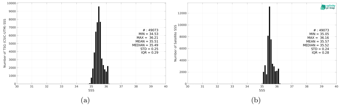
Figure 2: Histograms of SSS from TSG (CSIC-UTM) (a) and SMOS SSS L4 v1 - Monthly (CMEMS-CNR) (b) considering all match-up pairs per bins of 0.1 over the Indian Ocean Pi-MEP region and for the full satellite product period.
