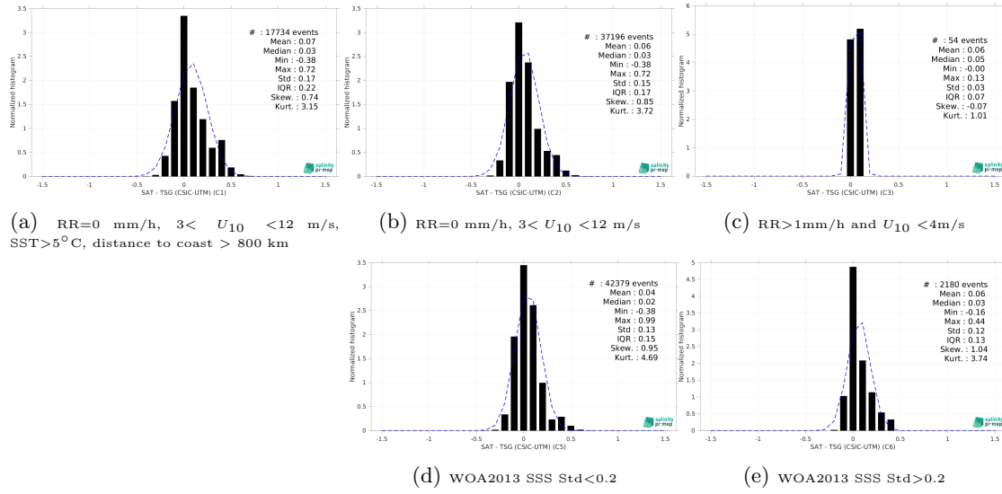
Figure 13: Normalized histogram of \Delta SSS (SMOS SSS L4 v1 - Monthly (CMEMS-CNR) - TSG (CSIC-UTM)) for 5 different subdatasets corresponding to: RR=0 mm/h, 3 < U_{10} < 12 m/s, SST>5°C, distance to coast > 800 km (a), RR=0 mm/h, 3 < U_{10} < 12 m/s (b), RR>1mm/h and U_{10} < 4 m/s (c), WOA2013 SSS Std<0.2 (d), WOA2013 SSS Std>0.2 (e).
