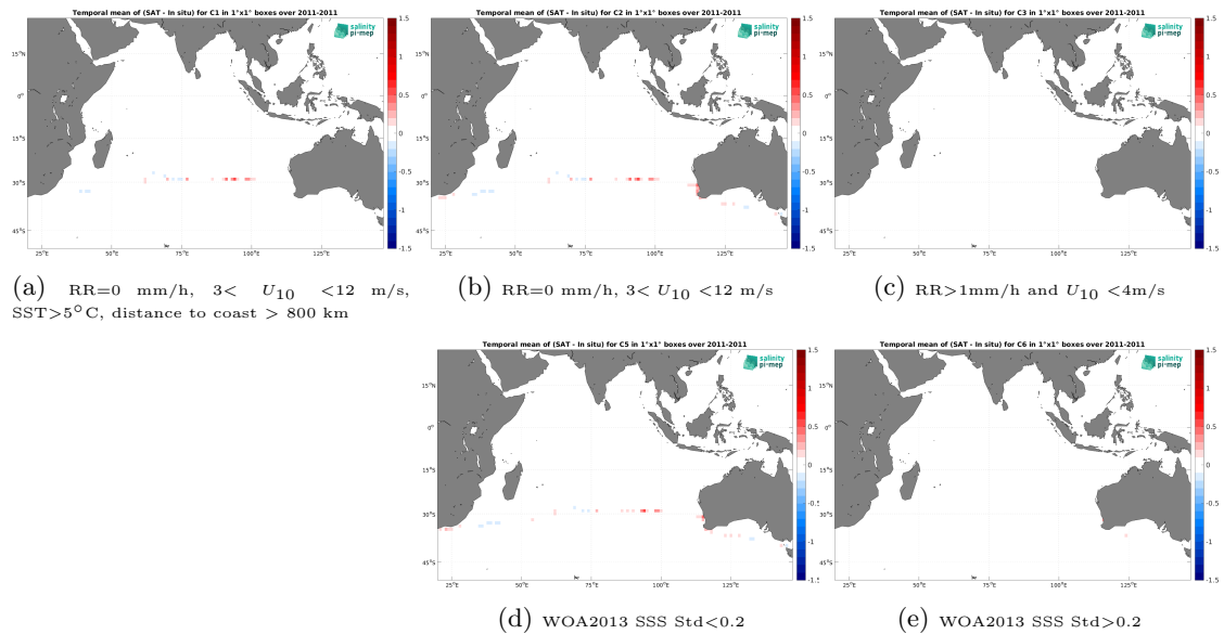
Figure 12: Temporal mean gridded over spatial boxes of size 1^\circ \times 1^\circ of \Delta SSS (SMOS SSS L4 v1 - Monthly (CMEMS-CNR) - TSG (CSIC-UTM)) for 5 different subdatasets corresponding to:RR=0 mm/h, 3 < U_{10} < 12 m/s, SST >5^\circ C, distance to coast > 800 km (a), RR=0 mm/h, 3 < U_{10} < 12 m/s (b), RR >1 mm/h and U_{10} < 4 m/s (c), WOA2013 SSS Std <0.2 (d), WOA2013 SSS Std >0.2 (e).
