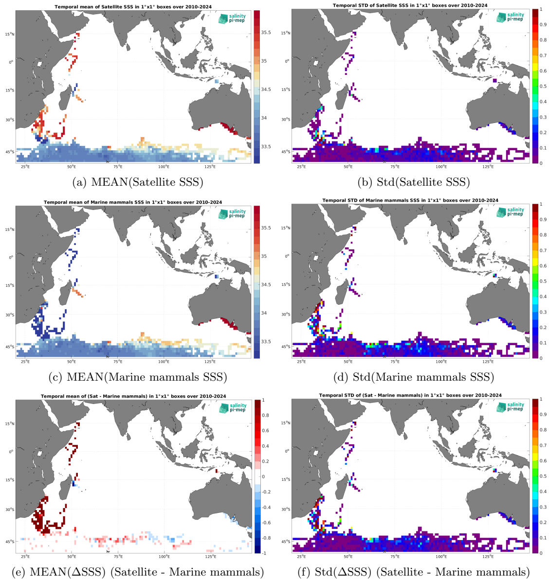
Figure 7: Temporal mean (left) and Std (right) of SSS from SMOS SSS L4 v1 - Monthly (CMEMS-CNR) (top), Marine mammals (middle), and of \Delta SSS (Satellite - Marine mammals). Only match-up pairs are used to generate these maps.
