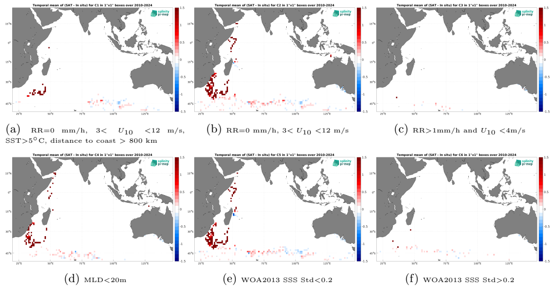
Figure 14: Temporal mean gridded over spatial boxes of size 1^\circ \times 1^\circ of \Delta SSS (SMOS SSS L4 v1 - Monthly (CMEMS-CNR) - Marine mammals) for 6 different subdatasets corresponding to:RR=0 mm/h, 3 < U_{10} < 12 m/s, SST > 5^\circ\text{C} , distance to coast > 800 km (a), RR=0 mm/h, 3 < U_{10} < 12 m/s (b), RR > 1 mm/h and U_{10} < 4 m/s (c),MLD < 20 m (d),WOA2013 SSS Std < 0.2 (e),WOA2013 SSS Std > 0.2 (f).
