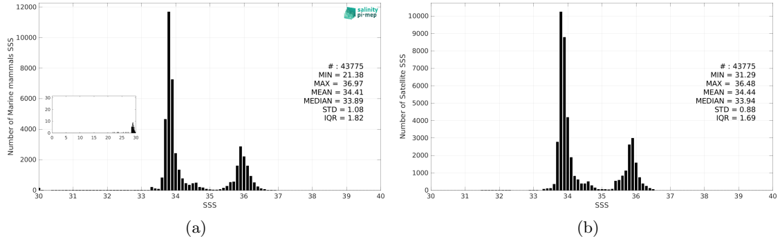
Figure 3: Histograms of SSS from Marine mammals (a) and SMOS SSS L4 v1 - Monthly (CMEMS-CNR) (b) considering all match-up pairs per bins of 0.1 over the Indian Ocean Pi-MEP region and for the full satellite product period.
