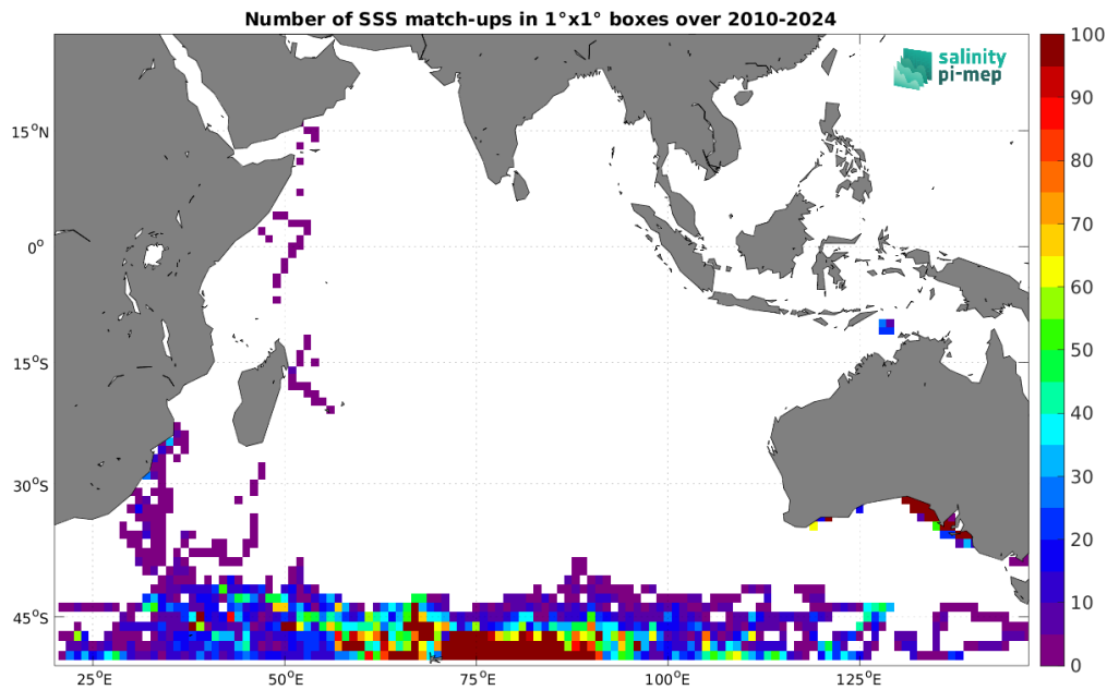
Figure 5: Number of SSS match-ups between Marine mammals SSS and the SMOS SSS L4 v1 - Monthly (CMEMS-CNR) SSS product for the Indian Ocean Pi-MEP region over 1^{\circ} \times 1^{\circ} boxes and for the full satellite product period.
