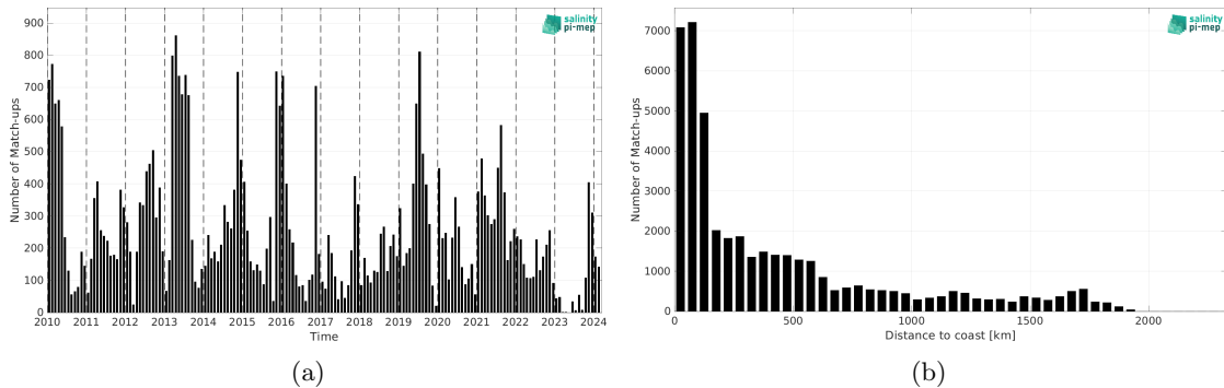
Figure 2: Number of match-ups between Marine mammals and SMOS SSS L4 v1 - Monthly (CMEMS-CNR) SSS as a function of time (a) and as function of the distance to coast (b) over the Indian Ocean Pi-MEP region and for the full satellite product period.
