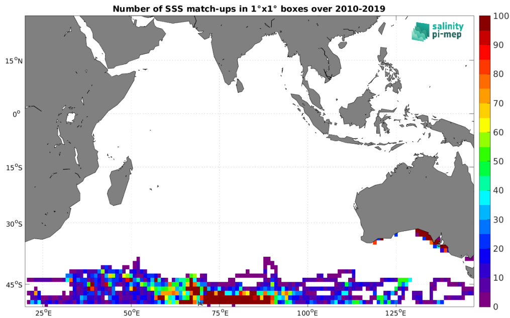
Figure 4: Number of SSS match-ups between Marine mammals SSS and the SMOS SSS L4 v1 - Monthly (CMEMS-CNR) SSS product for the Indian Ocean Pi-MEP region over 1^\circ \times 1^\circ boxes and for the full satellite product period.
