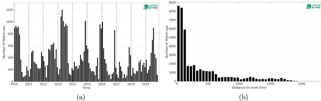
Figure 1: Number of match-ups between Marine mammals and SMOS SSS L4 v1 - Monthly (CMEMS-CNR) SSS as a function of time (a) and as function of the distance to coast (b) over the Indian Ocean Pi-MEP region and for the full satellite product period.
