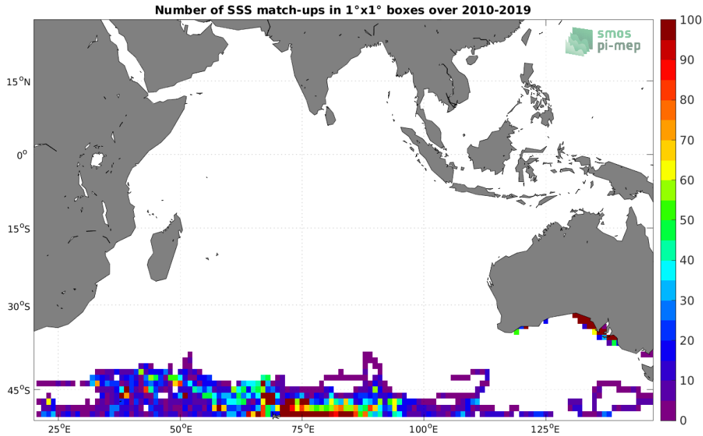
Figure 4: Number of SSS match-ups between Marine mammals SSS and the SMOS SSS L4 v1 - Monthly (CMEMS-CNR) SSS product for the Indian Ocean Pi-MEP region over 1^\circ \times 1^\circ boxes and for the full satellite product period.
