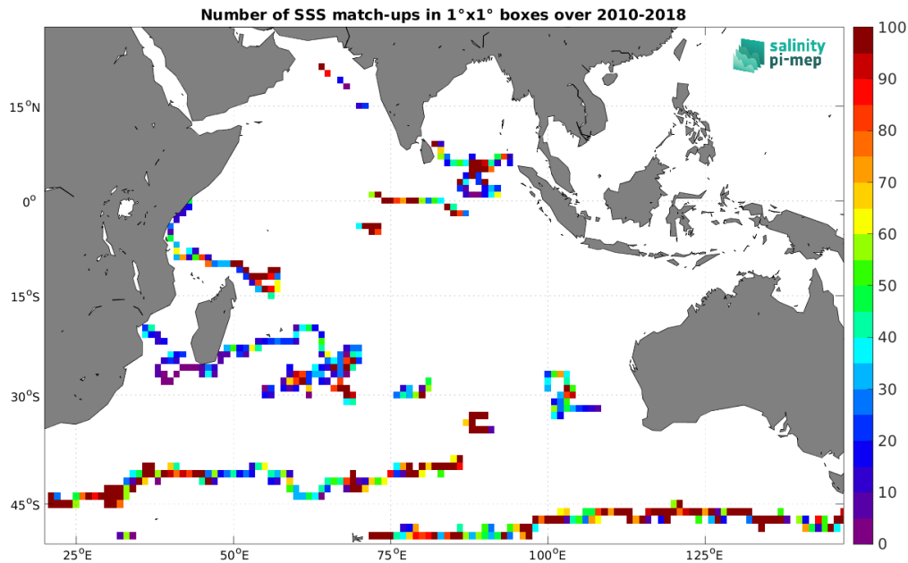
Figure 4: Number of SSS match-ups between Surface drifters SSS and the SMOS SSS L4 v1 - Monthly (CMEMS-CNR) SSS product for the Indian Ocean Pi-MEP region over 1^\circ \times 1^\circ boxes and for the full satellite product period.
