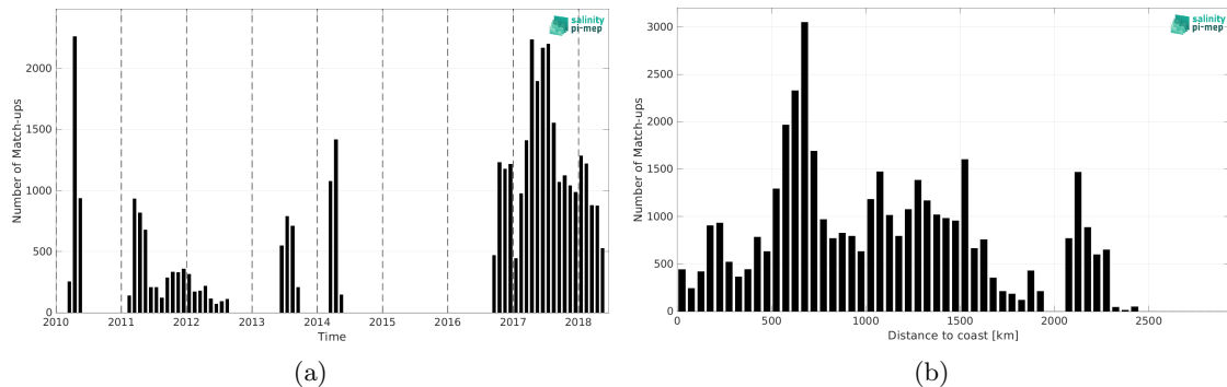
Figure 2: Number of match-ups between Surface drifters and SMOS SSS L4 v1 - Monthly (CMEMS-CNR) SSS as a function of time (a) and as function of the distance to coast (b) over the Indian Ocean Pi-MEP region and for the full satellite product period.
