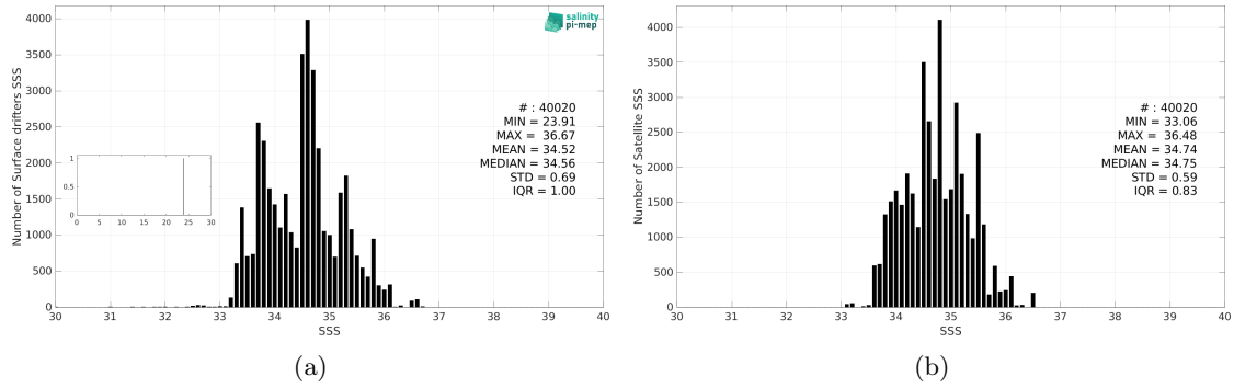
Figure 3: Histograms of SSS from Surface drifters (a) and SMOS SSS L4 v1 - Monthly (CMEMS-CNR) (b) considering all match-up pairs per bins of 0.1 over the Indian Ocean Pi-MEP region and for the full satellite product period.
