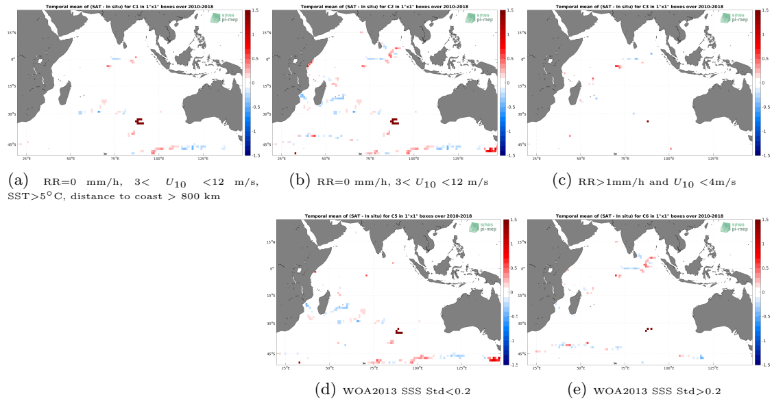
Figure 11: Temporal mean gridded over spatial boxes of size 1^\circ \times 1^\circ of \Delta SSS (SMOS SSS L4 v1 - Monthly (CMEMS-CNR) - Surface drifters) for 5 different subdatasets corresponding to:RR=0 mm/h, 3 < U_{10} < 12 m/s, SST >5^\circ C, distance to coast > 800 km (a), RR=0 mm/h, 3 < U_{10} < 12 m/s (b), RR >1 mm/h and U_{10} < 4 m/s (c), WOA2013 SSS Std <0.2 (d), WOA2013 SSS Std >0.2 (e).
