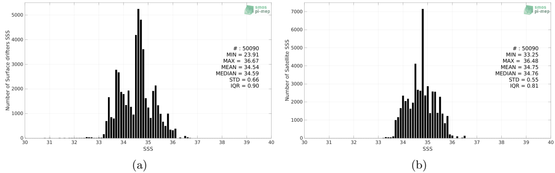
Figure 2: Histograms of SSS from Surface drifters (a) and SMOS SSS L4 v1 - Monthly (CMEMS-CNR) (b) considering all match-up pairs per bins of 0.1 over the Indian Ocean Pi-MEP region and for the full satellite product period.
