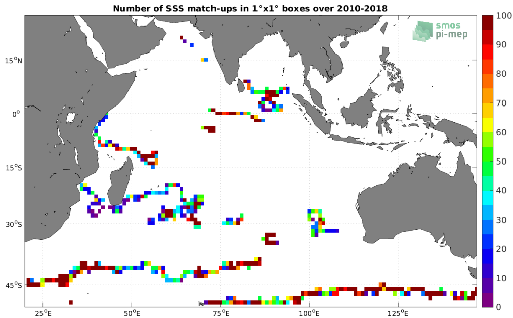
Figure 3: Number of SSS match-ups between Surface drifters SSS and the SMOS SSS L4 v1 - Monthly (CMEMS-CNR) SSS product for the Indian Ocean Pi-MEP region over 1^\circ \times 1^\circ boxes and for the full satellite product period.
