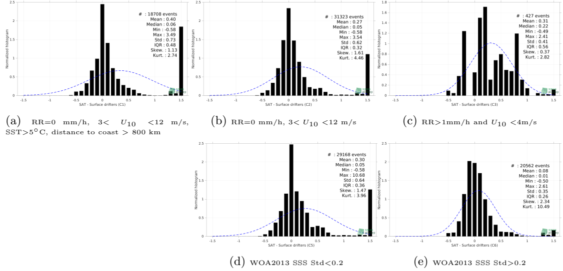
Figure 12: Normalized histogram of \Delta SSS (SMOS SSS L4 v1 - Monthly (CMEMS-CNR) - Surface drifters) for 5 different subdatasets corresponding to: RR=0 mm/h, 3 < U_{10} < 12 m/s, SST > 5°C, distance to coast > 800 km (a), RR=0 mm/h, 3 < U_{10} < 12 m/s (b), RR > 1mm/h and U_{10} < 4 m/s (c), WOA2013 SSS Std < 0.2 (d), WOA2013 SSS Std > 0.2 (e).
