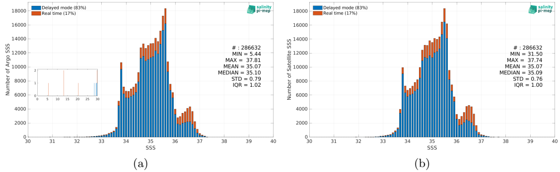
Figure 2: Histograms of SSS from Argo (a) and SMOS SSS L4 v1 - Monthly (CMEMS-CNR) (b) considering all match-up pairs per bins of 0.1 over the Indian Ocean Pi-MEP region and for the full satellite product period.
