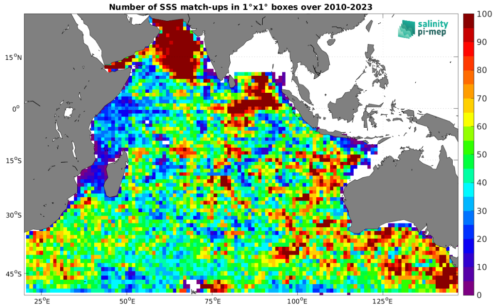
Figure 4: Number of SSS match-ups between Argo SSS and the SMOS SSS L4 v1 - Monthly (CMEMS-CNR) SSS product for the Indian Ocean Pi-MEP region over 1^\circ \times 1^\circ boxes and for the full satellite product period.
