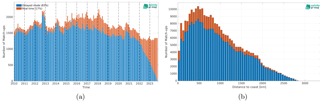
Figure 1: Number of match-ups between Argo and SMOS SSS L4 v1 - Monthly (CMEMS-CNR) SSS as a function of time (a) and as function of the distance to coast (b) over the Indian Ocean Pi-MEP region and for the full satellite product period.
