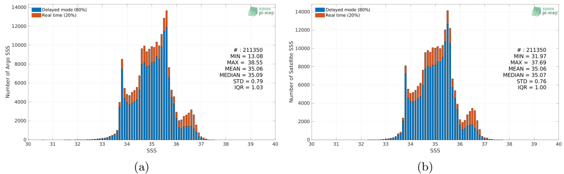
Figure 2: Histograms of SSS from Argo (a) and SMOS SSS L4 v1 - Monthly (CMEMS-CNR) (b) considering all match-up pairs per bins of 0.1 over the Indian Ocean Pi-MEP region and for the full satellite product period.
