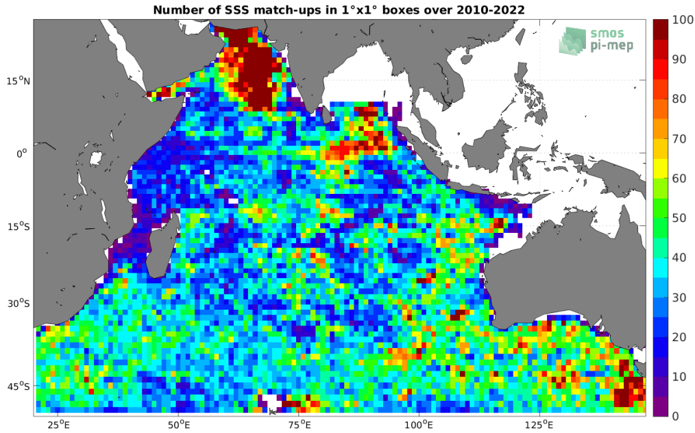
Figure 4: Number of SSS match-ups between Argo SSS and the SMOS SSS L4 v1 - Monthly (CMEMS-CNR) SSS product for the Indian Ocean Pi-MEP region over 1^\circ \times 1^\circ boxes and for the full satellite product period.
