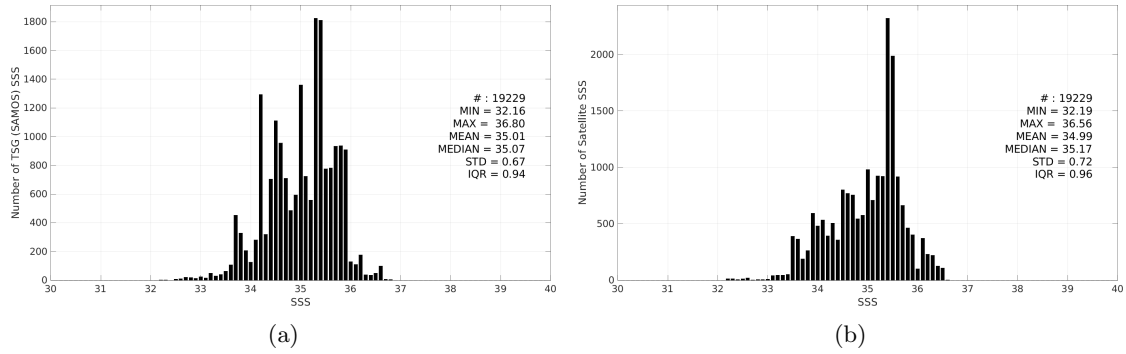
Figure 3: Histograms of SSS from TSG (SAMOS) (a) and SMOS SSS L4 v1 - Daily (CMEMS-CNR) (b) considering all match-up pairs per bins of 0.1 over the Indian Ocean Pi-MEP region and for the full satellite product period.
