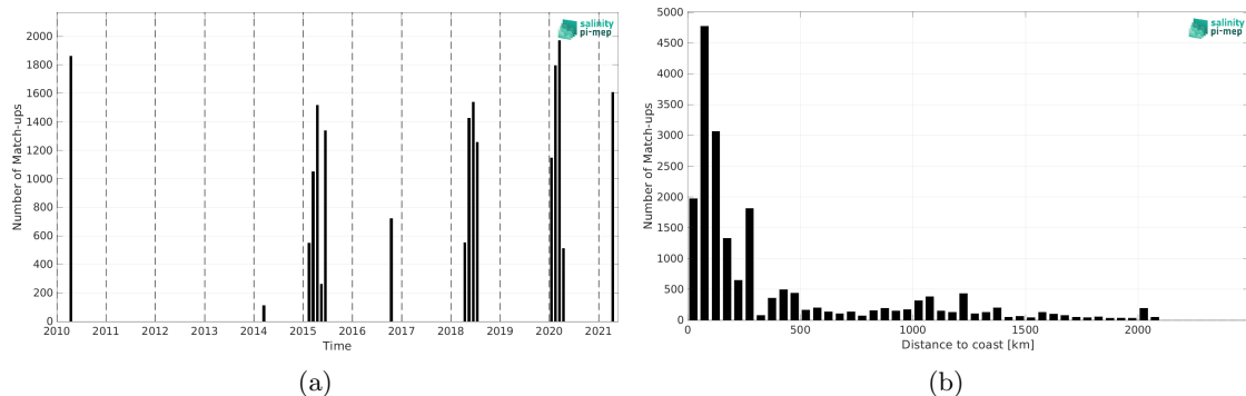
Figure 2: Number of match-ups between TSG (SAMOS) and SMOS SSS L4 v1 - Daily (CMEMS-CNR) SSS as a function of time (a) and as function of the distance to coast (b) over the Indian Ocean Pi-MEP region and for the full satellite product period.
