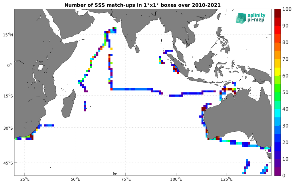
Figure 5: Number of SSS match-ups between TSG (SAMOS) SSS and the SMOS SSS L4 v1 - Daily (CMEMS-CNR) SSS product for the Indian Ocean Pi-MEP region over 1^\circ \times 1^\circ boxes and for the full satellite product period.
