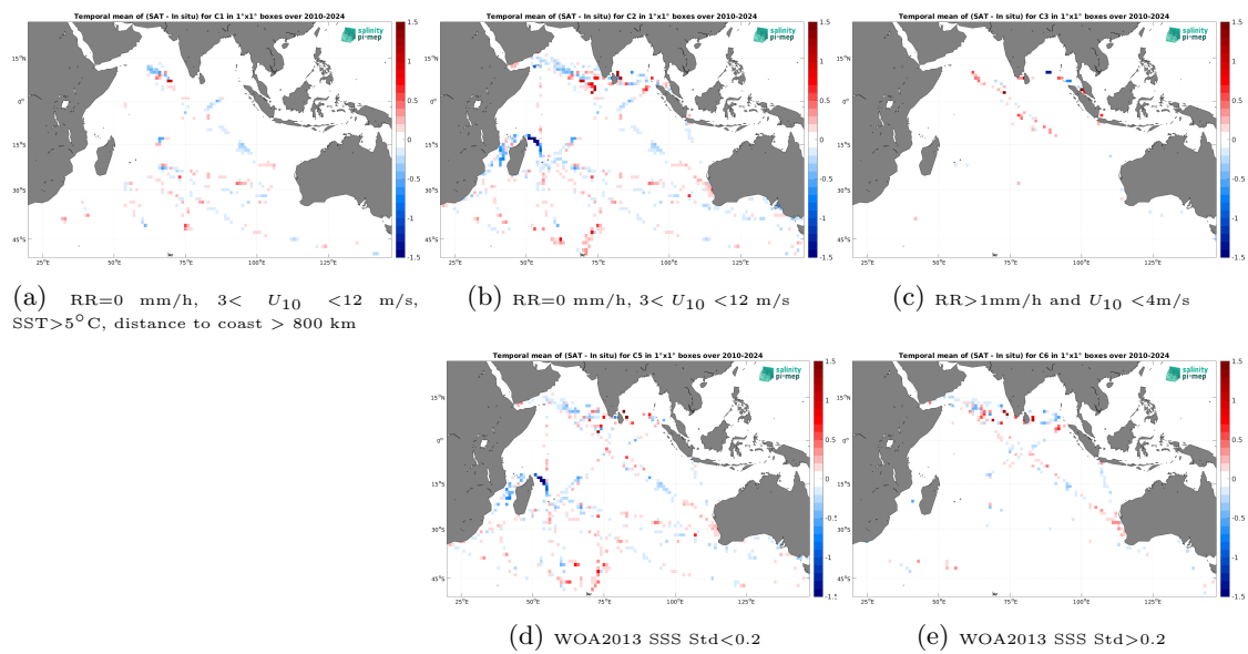
Figure 14: Temporal mean gridded over spatial boxes of size 1^\circ \times 1^\circ of \Delta SSS (SMOS SSS L4 v1 - Daily (CMEMS-CNR) - TSG (LEGOS-DM)) for 5 different subdatasets corresponding to: RR=0 mm/h, 3 < U_{10} < 12 m/s, SST > 5^\circ\text{C} , distance to coast > 800 km (a), RR=0 mm/h, 3 < U_{10} < 12 m/s (b), RR > 1 mm/h and U_{10} < 4 m/s (c), WOA2013 SSS Std < 0.2 (d), WOA2013 SSS Std > 0.2 (e).
