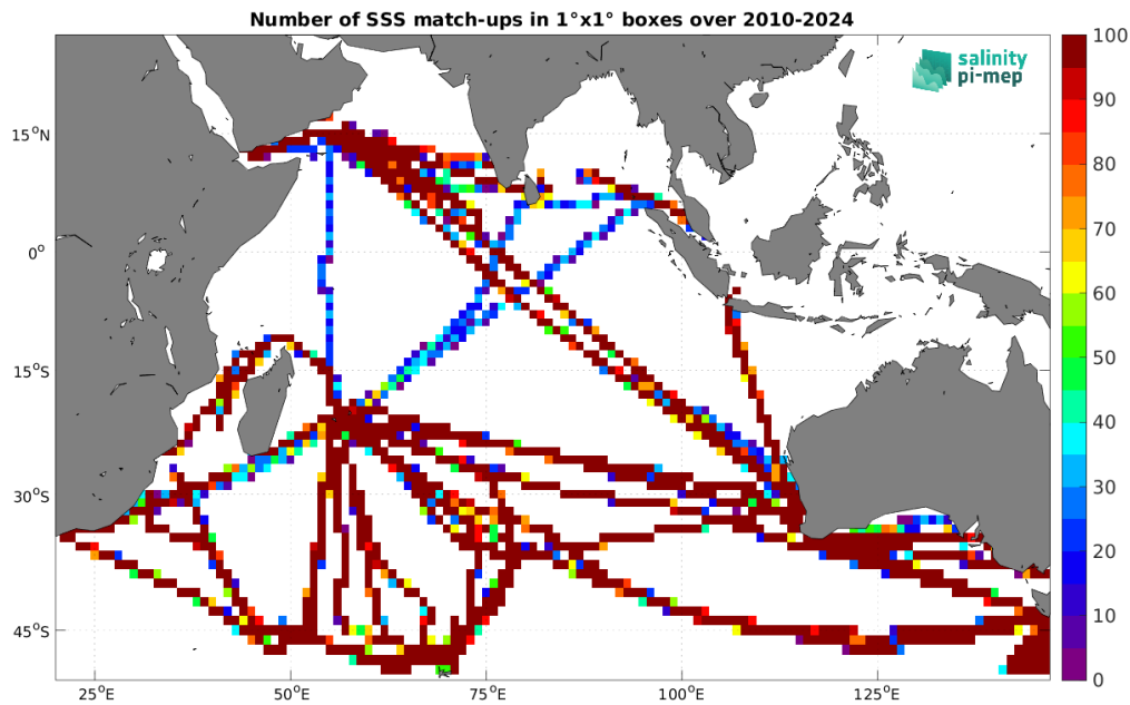
Figure 5: Number of SSS match-ups between TSG (LEGOS-DM) SSS and the SMOS SSS L4 v1 - Daily (CMEMS-CNR) SSS product for the Indian Ocean Pi-MEP region over 1^\circ \times 1^\circ boxes and for the full satellite product period.
