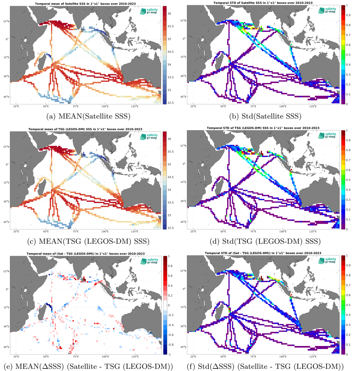
Figure 7: Temporal mean (left) and Std (right) of SSS from SMOS SSS L4 v1 - Daily (CMEMS-CNR) (top), TSG (LEGOS-DM) (middle), and of \Delta SSS (Satellite - TSG (LEGOS-DM)). Only match-up pairs are used to generate these maps.
