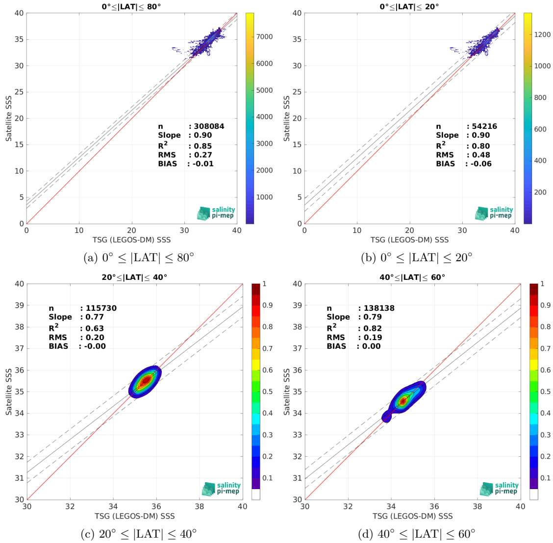
Figure 10: Contour maps of the concentration of SMOS SSS L4 v1 - Daily (CMEMS-CNR) SSS (y-axis) versus TSG (LEGOS-DM) SSS (x-axis) at match-up pairs for different latitude bands. For each plot, the red line shows x=y . The black thin and dashed lines indicate a linear fit through the data cloud and the \pm 95\% confidence levels, respectively. The number match-up pairs n , the slope and R^2 coefficient of the linear fit, the root mean square (RMS) and the mean bias between satellite and in situ data are indicated for each latitude band in each plots.
