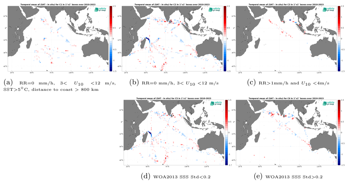
Figure 14: Temporal mean gridded over spatial boxes of size 1^\circ \times 1^\circ of \Delta SSS (SMOS SSS L4 v1 - Daily (CMEMS-CNR) - TSG (LEGOS-DM)) for 5 different subdatasets corresponding to:RR=0 mm/h, 3 < U_{10} < 12 m/s, SST > 5^\circ\text{C} , distance to coast > 800 km (a), RR=0 mm/h, 3 < U_{10} < 12 m/s (b), RR > 1 mm/h and U_{10} < 4 m/s (c), WOA2013 SSS Std < 0.2 (d), WOA2013 SSS Std > 0.2 (e).
