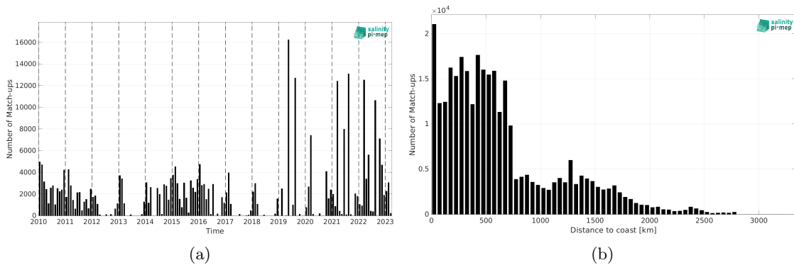
Figure 2: Number of match-ups between TSG (LEGOS-DM) and SMOS SSS L4 v1 - Daily (CMEMS-CNR) SSS as a function of time (a) and as function of the distance to coast (b) over the Indian Ocean Pi-MEP region and for the full satellite product period.
