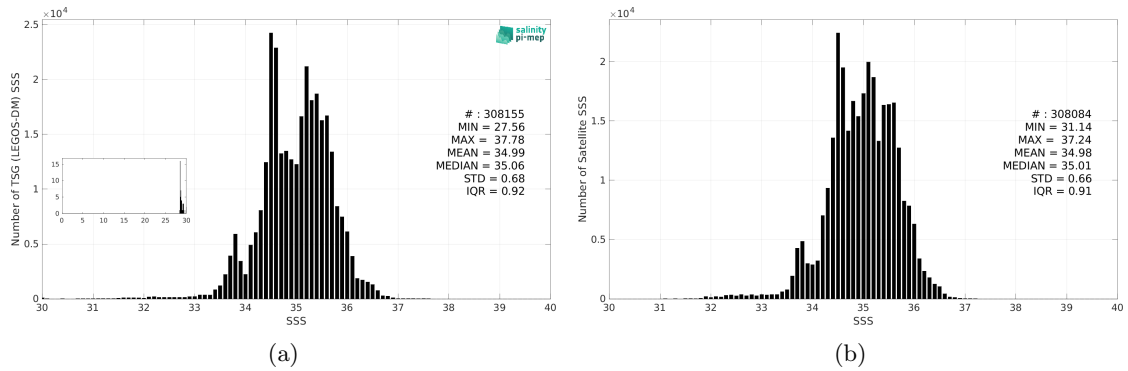
Figure 3: Histograms of SSS from TSG (LEGOS-DM) (a) and SMOS SSS L4 v1 - Daily (CMEMS-CNR) (b) considering all match-up pairs per bins of 0.1 over the Indian Ocean Pi-MEP region and for the full satellite product period.
