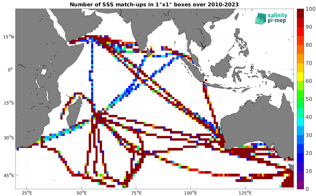
Figure 5: Number of SSS match-ups between TSG (LEGOS-DM) SSS and the SMOS SSS L4 v1 - Daily (CMEMS-CNR) SSS product for the Indian Ocean Pi-MEP region over 1^\circ \times 1^\circ boxes and for the full satellite product period.
