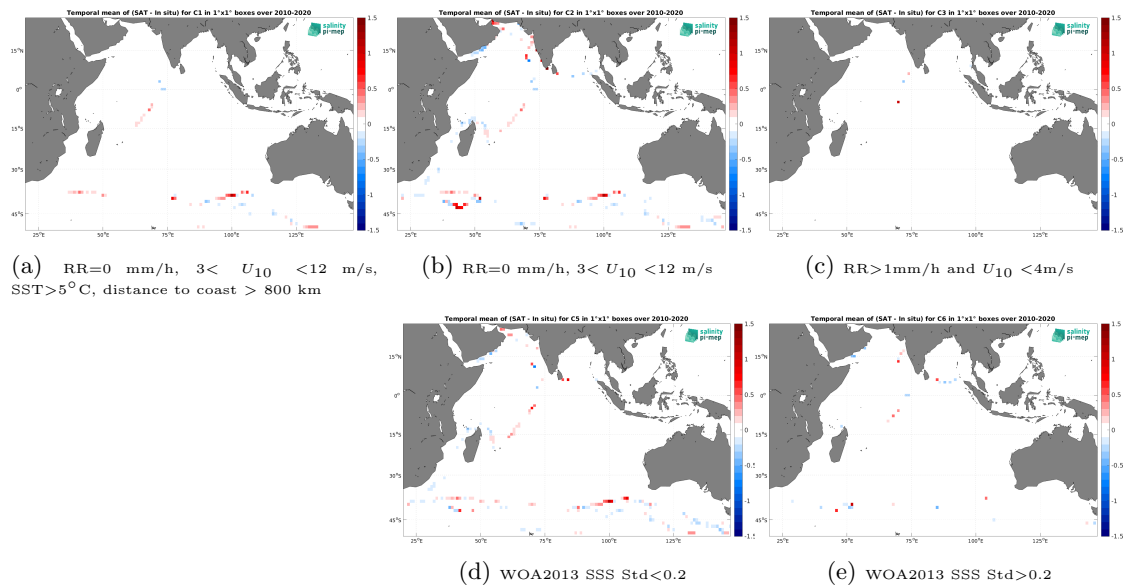
Figure 14: Temporal mean gridded over spatial boxes of size 1^\circ \times 1^\circ of \Delta SSS (SMOS SSS L4 v1 - Daily (CMEMS-CNR) - TSG (GOSUD-Sailing-ship)) for 5 different subdatasets corresponding to: RR=0 mm/h, 3 < U_{10} < 12 m/s, SST > 5^\circ\text{C} , distance to coast > 800 km (a), RR=0 mm/h, 3 < U_{10} < 12 m/s (b), RR > 1 mm/h and U_{10} < 4 m/s (c), WOA2013 SSS Std < 0.2 (d), WOA2013 SSS Std > 0.2 (e).
