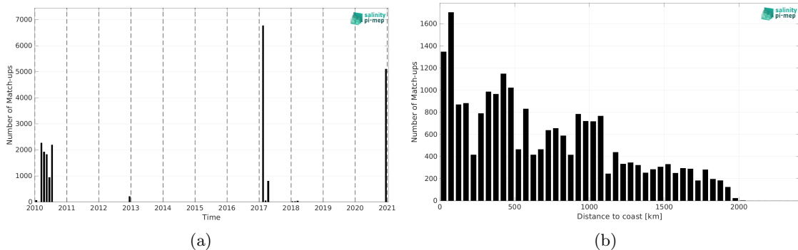
Figure 2: Number of match-ups between TSG (GOSUD-Sailing-ship) and SMOS SSS L4 v1 - Daily (CMEMS-CNR) SSS as a function of time (a) and as function of the distance to coast (b) over the Indian Ocean Pi-MEP region and for the full satellite product period.
