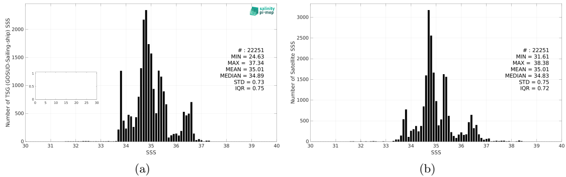
Figure 3: Histograms of SSS from TSG (GOSUD-Sailing-ship) (a) and SMOS SSS L4 v1 - Daily (CMEMS-CNR) (b) considering all match-up pairs per bins of 0.1 over the Indian Ocean Pi-MEP region and for the full satellite product period.
