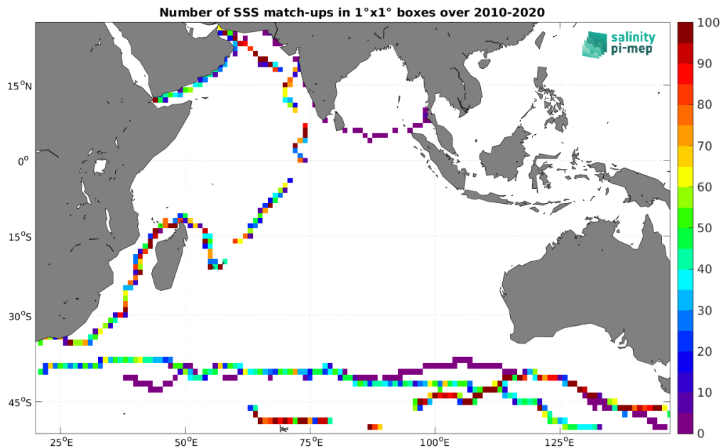
Figure 5: Number of SSS match-ups between TSG (GOSUD-Sailing-ship) SSS and the SMOS SSS L4 v1 - Daily (CMEMS-CNR) SSS product for the Indian Ocean Pi-MEP region over 1^\circ \times 1^\circ boxes and for the full satellite product period.
