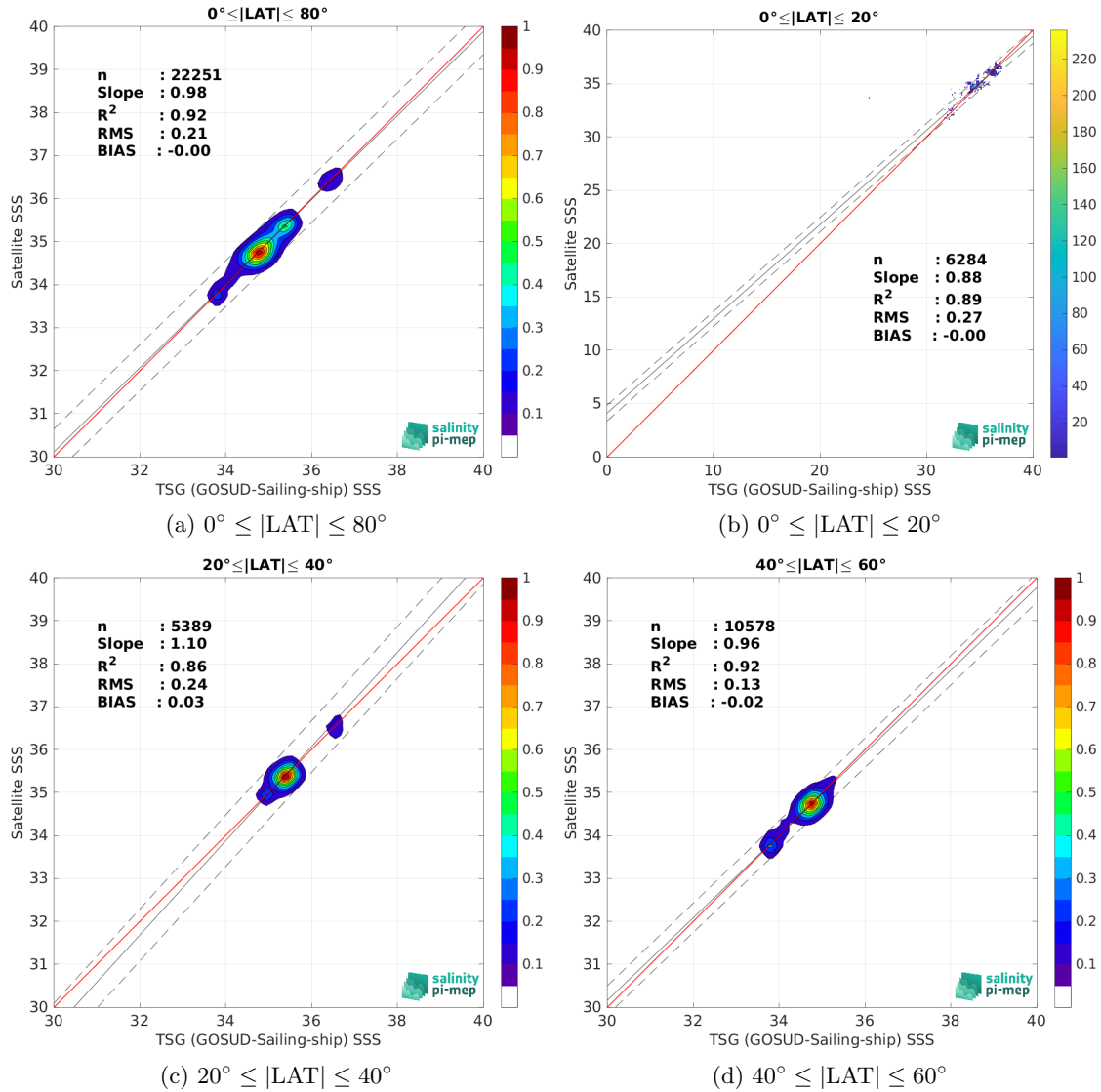
Figure 10: Contour maps of the concentration of SMOS SSS L4 v1 - Daily (CMEMS-CNR) SSS (y-axis) versus TSG (GOSUD-Sailing-ship) SSS (x-axis) at match-up pairs for different latitude bands. For each plot, the red line shows x=y . The black thin and dashed lines indicate a linear fit through the data cloud and the \pm 95\% confidence levels, respectively. The number match-up pairs n , the slope and R^2 coefficient of the linear fit, the root mean square (RMS) and the mean bias between satellite and in situ data are indicated for each latitude band in each plots.
