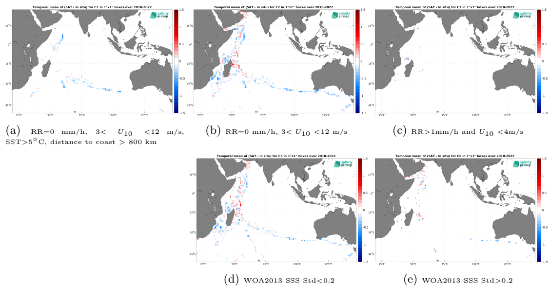
Figure 14: Temporal mean gridded over spatial boxes of size 1^\circ \times 1^\circ of \Delta SSS (SMOS SSS L4 v1 - Daily (CMEMS-CNR) - TSG (GOSUD-Research-vessel)) for 5 different subdatasets corresponding to:RR=0 mm/h, 3 < U_{10} < 12 m/s, SST > 5^\circ\text{C} , distance to coast > 800 km (a), RR=0 mm/h, 3 < U_{10} < 12 m/s (b), RR > 1 mm/h and U_{10} < 4 m/s (c), WOA2013 SSS Std < 0.2 (d), WOA2013 SSS Std > 0.2 (e).
