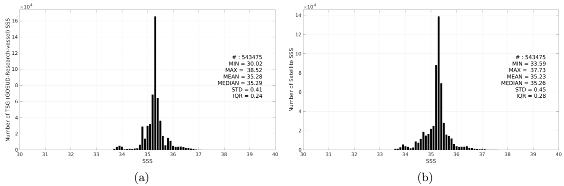
Figure 3: Histograms of SSS from TSG (GOSUD-Research-vessel) (a) and SMOS SSS L4 v1 - Daily (CMEMS-CNR) (b) considering all match-up pairs per bins of 0.1 over the Indian Ocean Pi-MEP region and for the full satellite product period.
