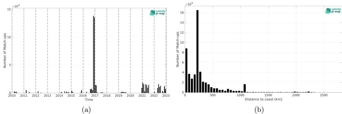
Figure 2: Number of match-ups between TSG (GOSUD-Research-vessel) and SMOS SSS L4 v1 - Daily (CMEMS-CNR) SSS as a function of time (a) and as function of the distance to coast (b) over the Indian Ocean Pi-MEP region and for the full satellite product period.
