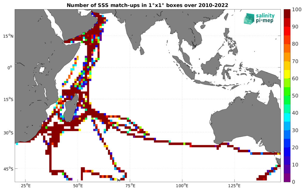
Figure 5: Number of SSS match-ups between TSG (GOSUD-Research-vessel) SSS and the SMOS SSS L4 v1 - Daily (CMEMS-CNR) SSS product for the Indian Ocean Pi-MEP region over 1^\circ \times 1^\circ boxes and for the full satellite product period.
