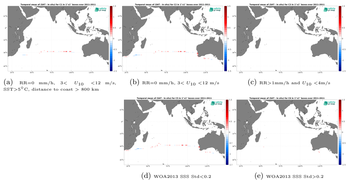
Figure 14: Temporal mean gridded over spatial boxes of size 1^\circ \times 1^\circ of \Delta SSS (SMOS SSS L4 v1 - Daily (CMEMS-CNR) - TSG (CSIC-UTM)) for 5 different subdatasets corresponding to:RR=0 mm/h, 3 < U_{10} < 12 m/s, SST >5^\circ\text{C} , distance to coast > 800 km (a), RR=0 mm/h, 3 < U_{10} < 12 m/s (b), RR >1 mm/h and U_{10} < 4 m/s (c), WOA2013 SSS Std <0.2 (d), WOA2013 SSS Std >0.2 (e).
