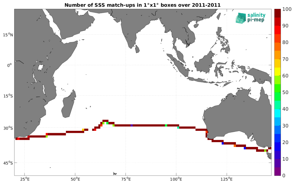
Figure 5: Number of SSS match-ups between TSG (CSIC-UTM) SSS and the SMOS SSS L4 v1 - Daily (CMEMS-CNR) SSS product for the Indian Ocean Pi-MEP region over 1^\circ \times 1^\circ boxes and for the full satellite product period.
