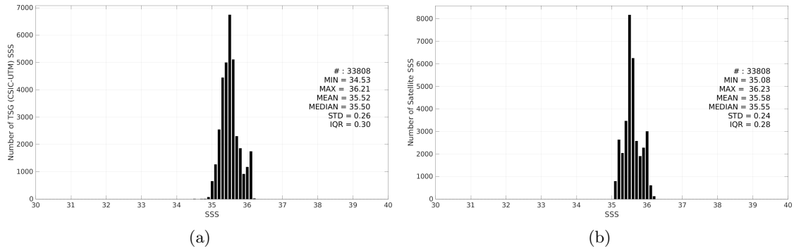
Figure 3: Histograms of SSS from TSG (CSIC-UTM) (a) and SMOS SSS L4 v1 - Daily (CMEMS-CNR) (b) considering all match-up pairs per bins of 0.1 over the Indian Ocean Pi-MEP region and for the full satellite product period.
