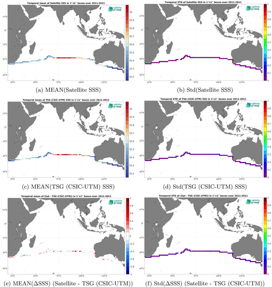
Figure 7: Temporal mean (left) and Std (right) of SSS from SMOS SSS L4 v1 - Daily (CMEMS-CNR) (top), TSG (CSIC-UTM) (middle), and of \Delta SSS (Satellite - TSG (CSIC-UTM)). Only match-up pairs are used to generate these maps.
