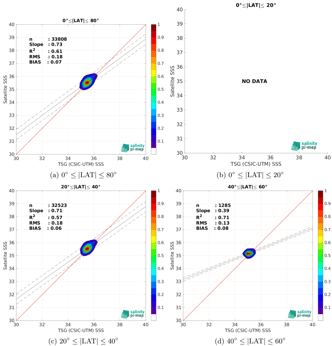
Figure 10: Contour maps of the concentration of SMOS SSS L4 v1 - Daily (CMEMS-CNR) SSS (y-axis) versus TSG (CSIC-UTM) SSS (x-axis) at match-up pairs for different latitude bands. For each plot, the red line shows x=y . The black thin and dashed lines indicate a linear fit through the data cloud and the \pm 95\% confidence levels, respectively. The number match-up pairs n , the slope and R^2 coefficient of the linear fit, the root mean square (RMS) and the mean bias between satellite and in situ data are indicated for each latitude band in each plots.
