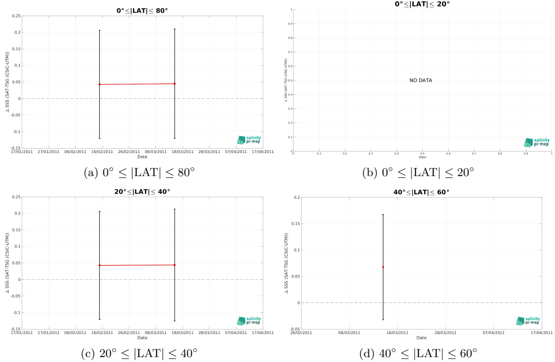
Figure 11: Monthly median (red curves) of \Delta\text{SSS} (Satellite - TSG (CSIC-UTM)) and \pm 1 Std (black vertical thick bars) as function of time for all the collected Pi-MEP match-up pairs estimated over the Indian Ocean Pi-MEP region and for the full satellite product period are shown for different latitude bands: (a) 80^{\circ}\text{S}-80^{\circ}\text{N} , (b) 20^{\circ}\text{S}-20^{\circ}\text{N} , (c) 40^{\circ}\text{S}-20^{\circ}\text{S} and 20^{\circ}\text{N}-40^{\circ}\text{N} and (d) 60^{\circ}\text{S}-40^{\circ}\text{S} and 40^{\circ}\text{N}-60^{\circ}\text{N} .
