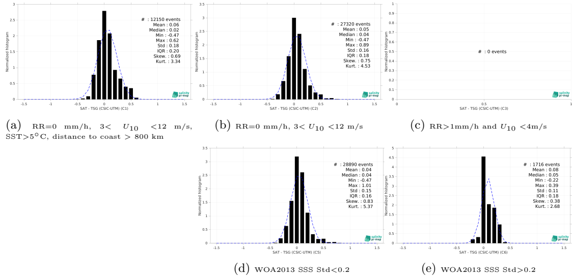
Figure 15: Normalized histogram of \Delta SSS (SMOS SSS L4 v1 - Daily (CMEMS-CNR) - TSG (CSIC-UTM)) for 5 different subdatasets corresponding to: RR=0 mm/h, 3 < U_{10} < 12 m/s, SST > 5°C, distance to coast > 800 km (a), RR=0 mm/h, 3 < U_{10} < 12 m/s (b), RR > 1mm/h and U_{10} < 4 m/s (c), WOA2013 SSS Std < 0.2 (d), WOA2013 SSS Std > 0.2 (e).
