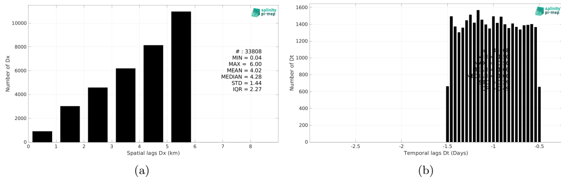
Figure 6: Histograms of the spatial (a) and temporal (b) lags between the location/time of the TSG (CSIC-UTM) measurement and the date of the corresponding SMOS SSS L4 v1 - Daily (CMEMS-CNR) SSS pixel.
