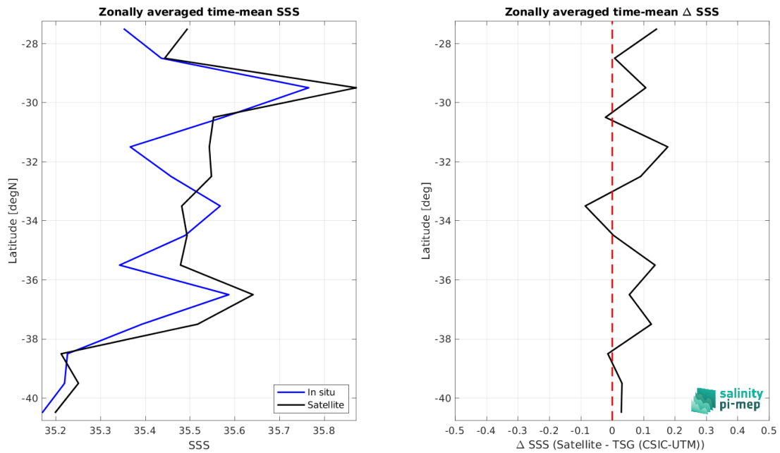
Figure 9: Left panel: Zonal mean SSS from SMOS SSS L4 v1 - Daily (CMEMS-CNR) satellite product (black) and from TSG (CSIC-UTM) (blue). Right panel: Zonal mean of \Delta SSS (Satellite - TSG (CSIC-UTM)) for all the collected Pi-MEP match-up pairs estimated over the full satellite product period.
