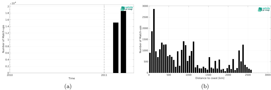
Figure 2: Number of match-ups between TSG (CSIC-UTM) and SMOS SSS L4 v1 - Daily (CMEMS-CNR) SSS as a function of time (a) and as function of the distance to coast (b) over the Indian Ocean Pi-MEP region and for the full satellite product period.
