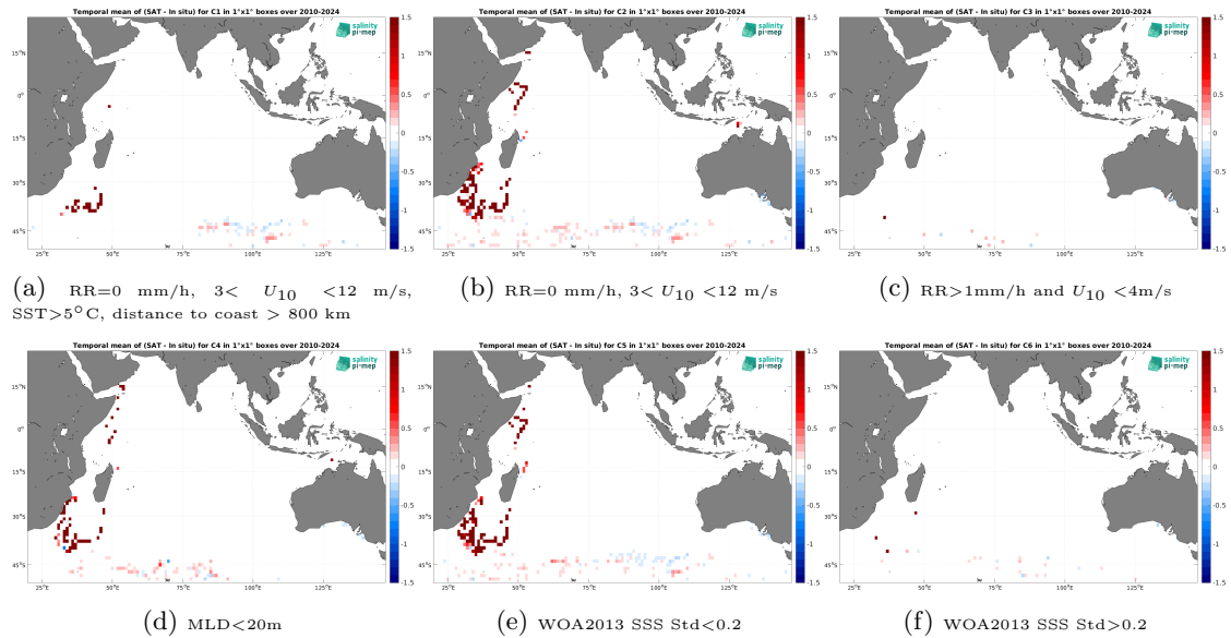
Figure 14: Temporal mean gridded over spatial boxes of size 1^\circ \times 1^\circ of \Delta SSS (SMOS SSS L4 v1 - Daily (CMEMS-CNR) - Marine mammals) for 6 different subdatasets corresponding to: RR=0 mm/h, 3 < U_{10} < 12 m/s, SST > 5°C, distance to coast > 800 km (a), RR=0 mm/h, 3 < U_{10} < 12 m/s (b), RR > 1mm/h and U_{10} < 4 m/s (c), MLD < 20m (d), WOA2013 SSS Std < 0.2 (e), WOA2013 SSS Std > 0.2 (f).
