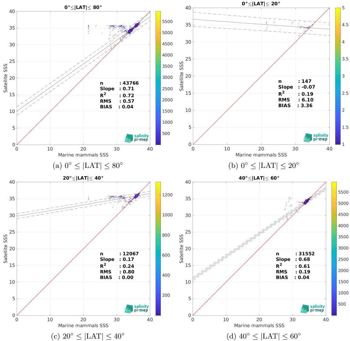
Figure 10: Contour maps of the concentration of SMOS SSS L4 v1 - Daily (CMEMS-CNR) SSS (y-axis) versus Marine mammals SSS (x-axis) at match-up pairs for different latitude bands. For each plot, the red line shows x=y . The black thin and dashed lines indicate a linear fit through the data cloud and the \pm 95\% confidence levels, respectively. The number match-up pairs n , the slope and R^2 coefficient of the linear fit, the root mean square (RMS) and the mean bias between satellite and in situ data are indicated for each latitude band in each plots.
