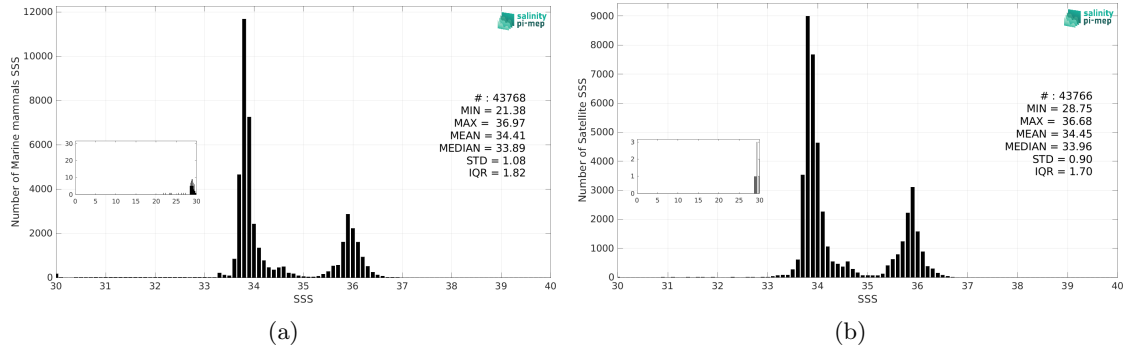
Figure 3: Histograms of SSS from Marine mammals (a) and SMOS SSS L4 v1 - Daily (CMEMS-CNR) (b) considering all match-up pairs per bins of 0.1 over the Indian Ocean Pi-MEP region and for the full satellite product period.
