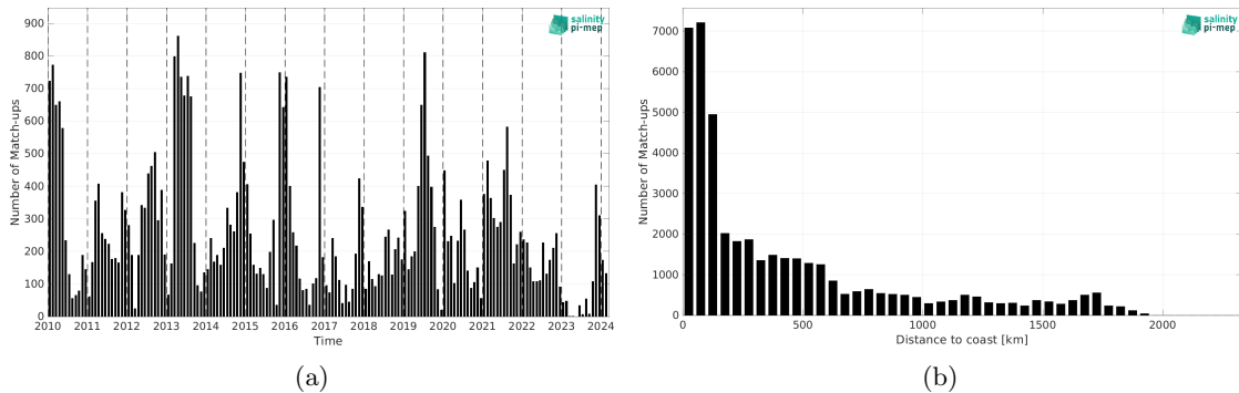
Figure 2: Number of match-ups between Marine mammals and SMOS SSS L4 v1 - Daily (CMEMS-CNR) SSS as a function of time (a) and as function of the distance to coast (b) over the Indian Ocean Pi-MEP region and for the full satellite product period.
