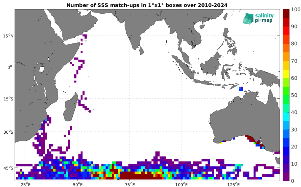
Figure 5: Number of SSS match-ups between Marine mammals SSS and the SMOS SSS L4 v1 - Daily (CMEMS-CNR) SSS product for the Indian Ocean Pi-MEP region over 1^\circ \times 1^\circ boxes and for the full satellite product period.
