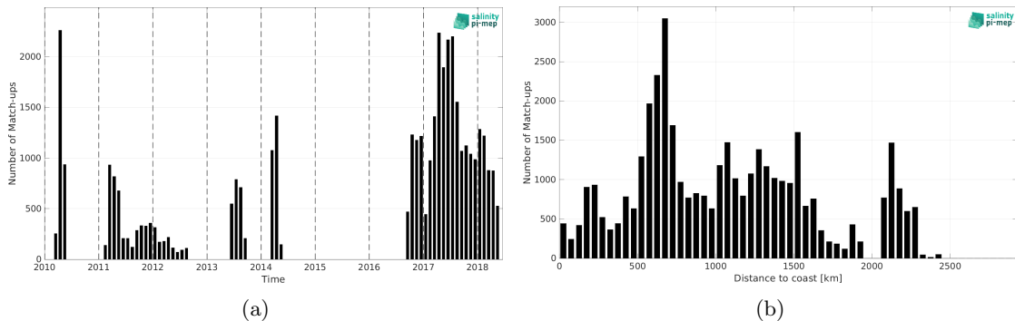
Figure 2: Number of match-ups between Surface drifters and SMOS SSS L4 v1 - Daily (CMEMS-CNR) SSS as a function of time (a) and as function of the distance to coast (b) over the Indian Ocean Pi-MEP region and for the full satellite product period.
