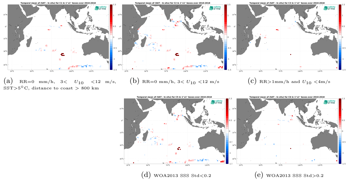
Figure 13: Temporal mean gridded over spatial boxes of size 1^\circ \times 1^\circ of \Delta SSS (SMOS SSS L4 v1 - Daily (CMEMS-CNR) - Surface drifters) for 5 different subdatasets corresponding to: RR=0 mm/h, 3 < U_{10} < 12 m/s, SST > 5^\circ\text{C} , distance to coast > 800 km (a), RR=0 mm/h, 3 < U_{10} < 12 m/s (b), RR > 1 mm/h and U_{10} < 4 m/s (c), WOA2013 SSS Std < 0.2 (d), WOA2013 SSS Std > 0.2 (e).
