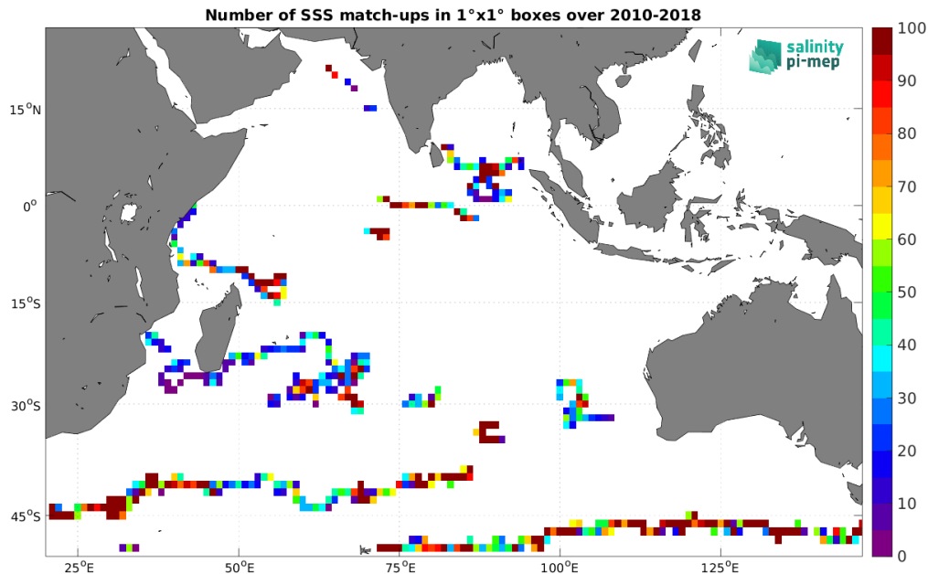
Figure 4: Number of SSS match-ups between Surface drifters SSS and the SMOS SSS L4 v1 - Daily (CMEMS-CNR) SSS product for the Indian Ocean Pi-MEP region over 1^\circ \times 1^\circ boxes and for the full satellite product period.
