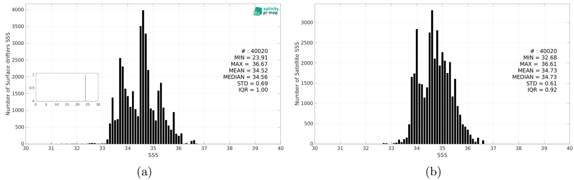
Figure 3: Histograms of SSS from Surface drifters (a) and SMOS SSS L4 v1 - Daily (CMEMS-CNR) (b) considering all match-up pairs per bins of 0.1 over the Indian Ocean Pi-MEP region and for the full satellite product period.
