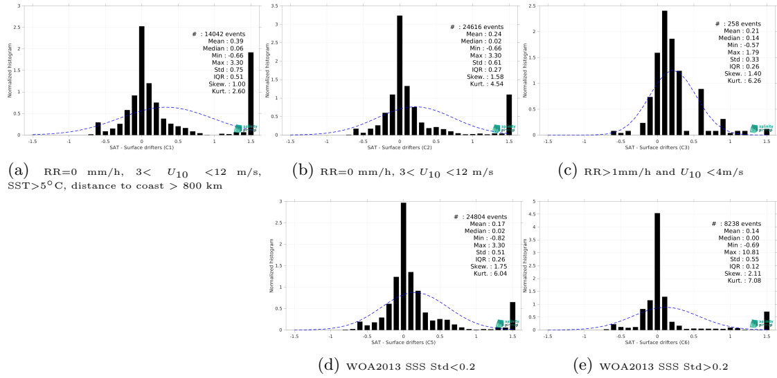
Figure 14: Normalized histogram of \Delta SSS (SMOS SSS L4 v1 - Daily (CMEMS-CNR) - Surface drifters) for 5 different subdatasets corresponding to: RR=0 mm/h, 3 < U_{10} < 12 m/s, SST >5^{\circ} C, distance to coast > 800 km (a), RR=0 mm/h, 3 < U_{10} < 12 m/s (b), RR >1 mm/h and U_{10} < 4 m/s (c), WOA2013 SSS Std <0.2 (d), WOA2013 SSS Std >0.2 (e).
