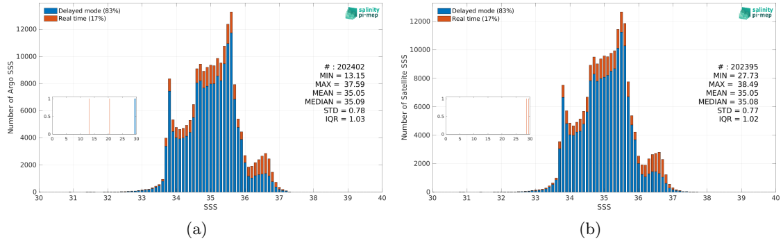
Figure 3: Histograms of SSS from Argo (a) and SMOS SSS L4 v1 - Daily (CMEMS-CNR) (b) considering all match-up pairs per bins of 0.1 over the Indian Ocean Pi-MEP region and for the full satellite product period.
