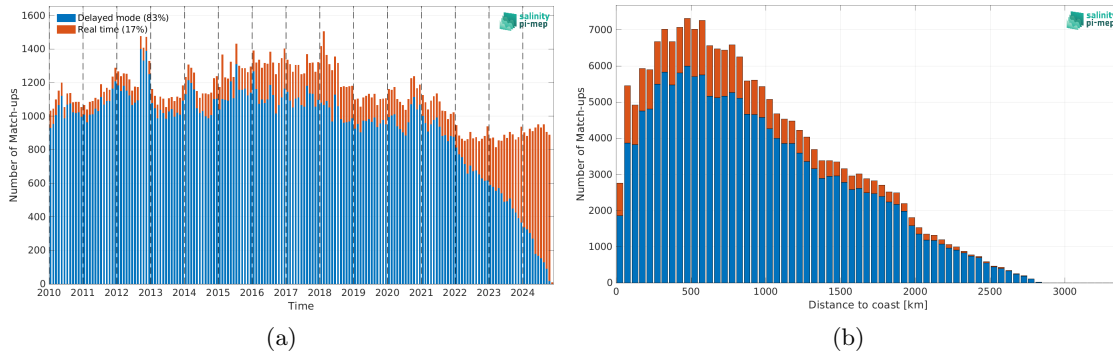
Figure 2: Number of match-ups between Argo and SMOS SSS L4 v1 - Daily (CMEMS-CNR) SSS as a function of time (a) and as function of the distance to coast (b) over the Indian Ocean Pi-MEP region and for the full satellite product period.
