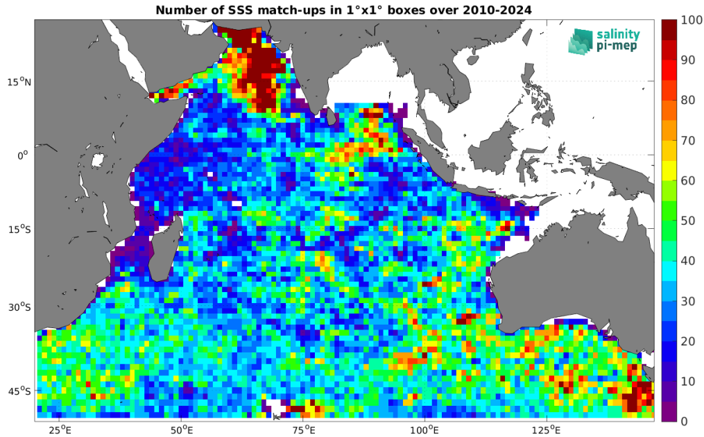
Figure 5: Number of SSS match-ups between Argo SSS and the SMOS SSS L4 v1 - Daily (CMEMS-CNR) SSS product for the Indian Ocean Pi-MEP region over 1^\circ \times 1^\circ boxes and for the full satellite product period.
