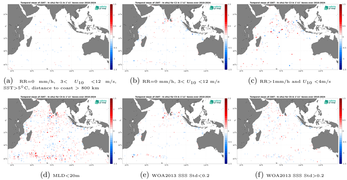
Figure 14: Temporal mean gridded over spatial boxes of size 1^\circ \times 1^\circ of \Delta\text{SSS} (SMOS SSS L4 v1 - Daily (CMEMS-CNR) - Argo) for 6 different subdatasets corresponding to:RR=0 mm/h, 3 < U_{10} < 12 m/s, SST>5°C, distance to coast > 800 km (a), RR=0 mm/h, 3 < U_{10} < 12 m/s (b), RR>1mm/h and U_{10} < 4 m/s (c),MLD<20m (d),WOA2013 SSS Std<0.2 (e),WOA2013 SSS Std>0.2 (f).
