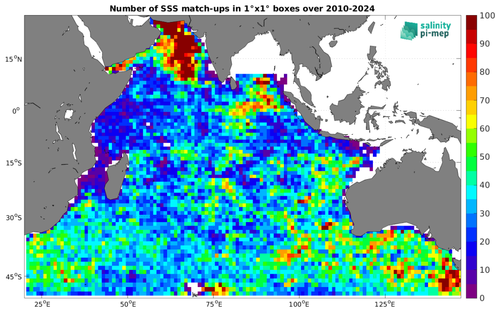
Figure 5: Number of SSS match-ups between Argo SSS and the SMOS SSS L4 v1 - Daily (CMEMS-CNR) SSS product for the Indian Ocean Pi-MEP region over 1^\circ \times 1^\circ boxes and for the full satellite product period.
