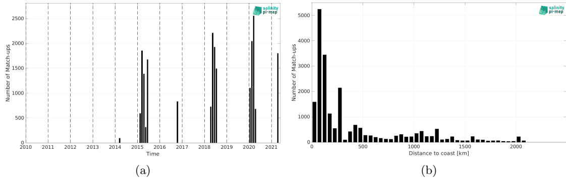
Figure 2: Number of match-ups between TSG (SAMOS) and SMOS SSS L4 OI v346 - Weekly (CMEMS-CATDS-LOPS) SSS as a function of time (a) and as function of the distance to coast (b) over the Indian Ocean Pi-MEP region and for the full satellite product period.
