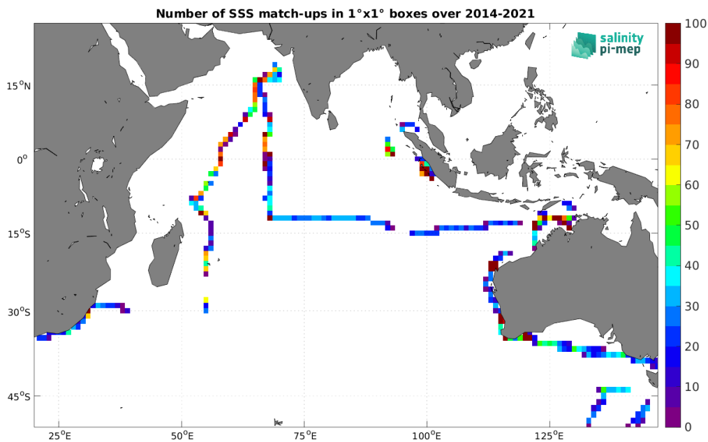
Figure 5: Number of SSS match-ups between TSG (SAMOS) SSS and the SMOS SSS L4 OI v346 - Weekly (CMEMS-CATDS-LOPS) SSS product for the Indian Ocean Pi-MEP region over 1^\circ \times 1^\circ boxes and for the full satellite product period.
