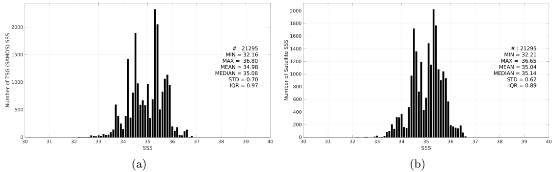
Figure 3: Histograms of SSS from TSG (SAMOS) (a) and SMOS SSS L4 OI v346 - Weekly (CMEMS-CATDS-LOPS) (b) considering all match-up pairs per bins of 0.1 over the Indian Ocean Pi-MEP region and for the full satellite product period.
