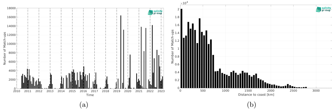
Figure 2: Number of match-ups between TSG (LEGOS-DM) and SMOS SSS L4 OI v346 - Weekly (CMEMS-CATDS-LOPS) SSS as a function of time (a) and as function of the distance to coast (b) over the Indian Ocean Pi-MEP region and for the full satellite product period.
