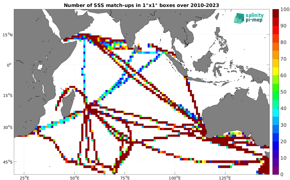
Figure 5: Number of SSS match-ups between TSG (LEGOS-DM) SSS and the SMOS SSS L4 OI v346 - Weekly (CMEMS-CATDS-LOPS) SSS product for the Indian Ocean Pi-MEP region over 1^\circ \times 1^\circ boxes and for the full satellite product period.
