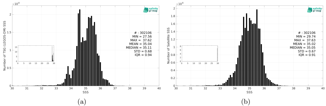
Figure 3: Histograms of SSS from TSG (LEGOS-DM) (a) and SMOS SSS L4 OI v346 - Weekly (CMEMS-CATDS-LOPS) (b) considering all match-up pairs per bins of 0.1 over the Indian Ocean Pi-MEP region and for the full satellite product period.
