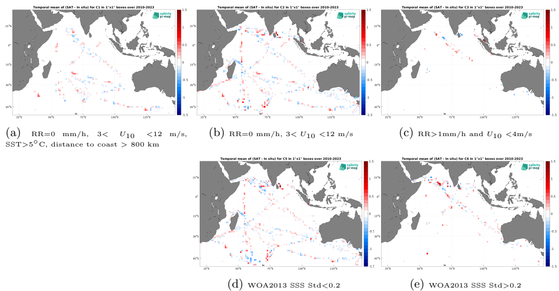
Figure 14: Temporal mean gridded over spatial boxes of size 1^\circ \times 1^\circ of \Delta SSS (SMOS SSS L4 OI v346 - Weekly (CMEMS-CATDS-LOPS) - TSG (LEGOS-DM)) for 5 different subdatasets corresponding to:RR=0 mm/h, 3 < U_{10} < 12 m/s, SST >5^\circ\text{C} , distance to coast > 800 km (a), RR=0 mm/h, 3 < U_{10} < 12 m/s (b), RR >1 mm/h and U_{10} < 4 m/s (c), WOA2013 SSS Std <0.2 (d), WOA2013 SSS Std >0.2 (e).
