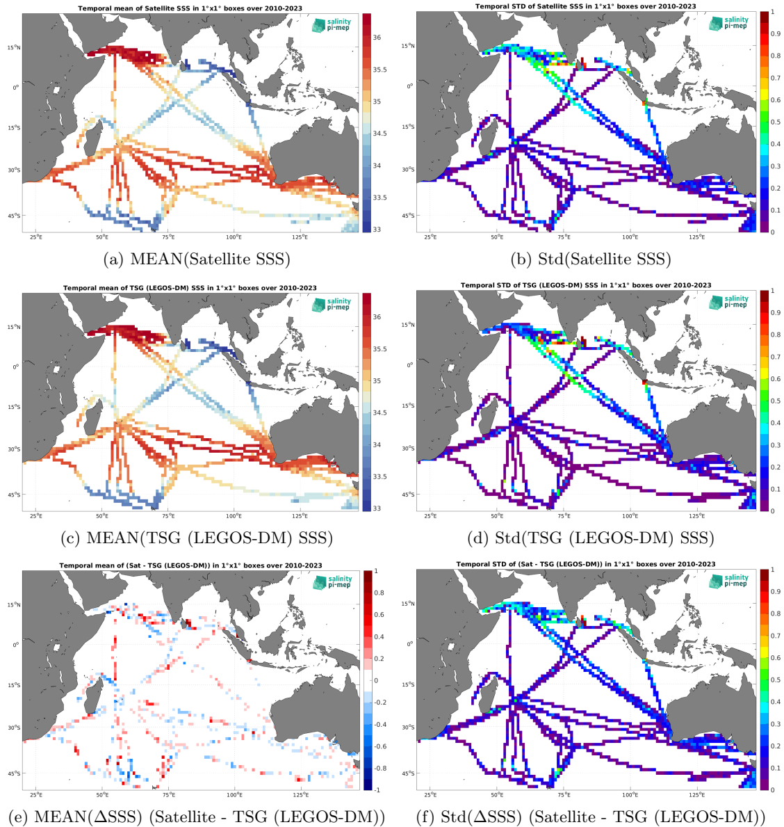
Figure 7: Temporal mean (left) and Std (right) of SSS from SMOS SSS L4 OI v346 - Weekly (CMEMS-CATDS-LOPS) (top), TSG (LEGOS-DM) (middle), and of \Delta SSS (Satellite - TSG (LEGOS-DM)). Only match-up pairs are used to generate these maps.
