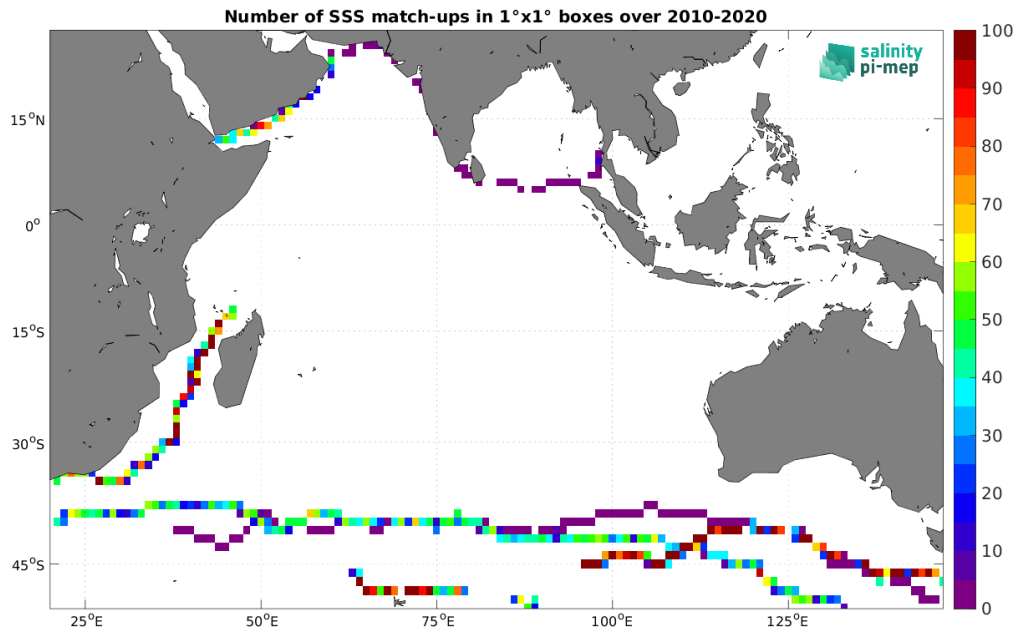
Figure 5: Number of SSS match-ups between TSG (GOSUD-Sailing-ship) SSS and the SMOS SSS L4 OI v346 - Weekly (CMEMS-CATDS-LOPS) SSS product for the Indian Ocean Pi-MEP region over 1^\circ \times 1^\circ boxes and for the full satellite product period.
