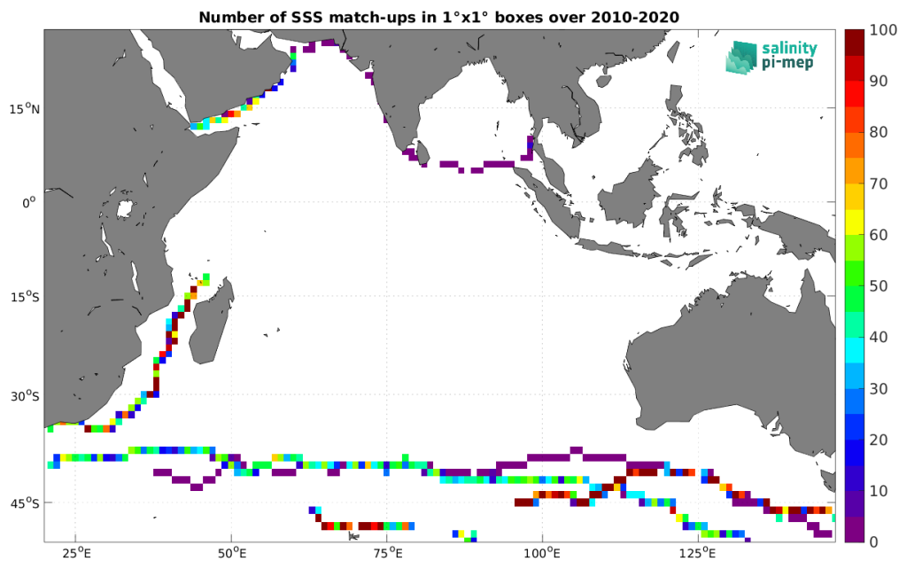
Figure 5: Number of SSS match-ups between TSG (GOSUD-Sailing-ship) SSS and the SMOS SSS L4 OI v346 - Weekly (CMEMS-CATDS-LOPS) SSS product for the Indian Ocean Pi-MEP region over 1^\circ \times 1^\circ boxes and for the full satellite product period.
