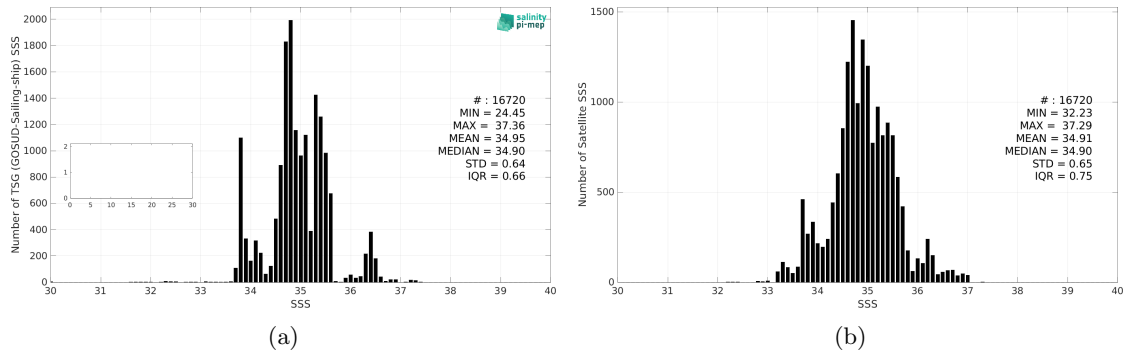
Figure 3: Histograms of SSS from TSG (GOSUD-Sailing-ship) (a) and SMOS SSS L4 OI v346 - Weekly (CMEMS-CATDS-LOPS) (b) considering all match-up pairs per bins of 0.1 over the Indian Ocean Pi-MEP region and for the full satellite product period.
