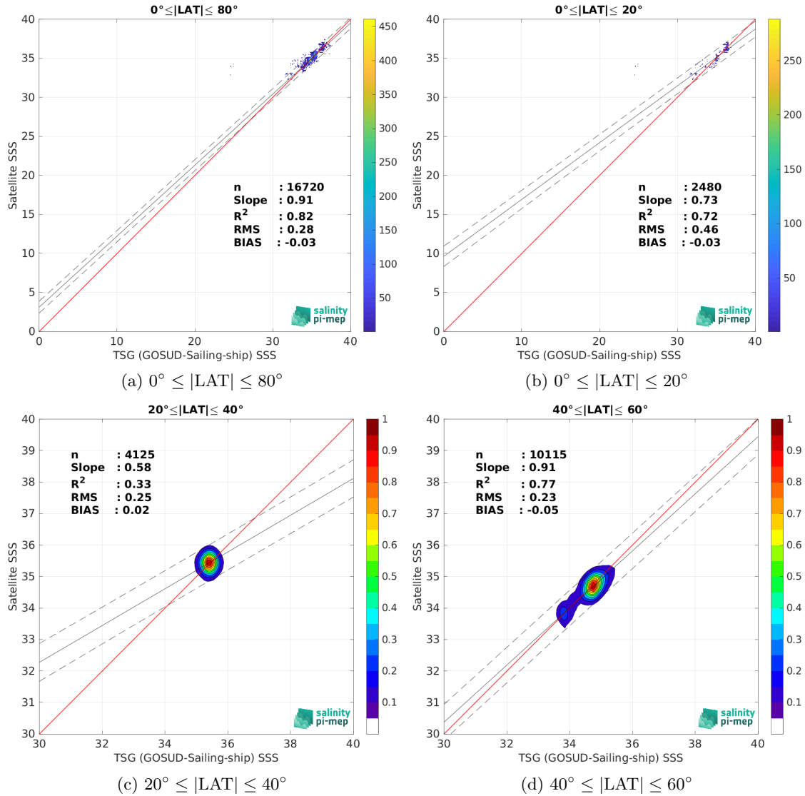
Figure 10: Contour maps of the concentration of SMOS SSS L4 OI v346 - Weekly (CMEMS-CATDS-LOPS) SSS ( y -axis) versus TSG (GOSUD-Sailing-ship) SSS ( x -axis) at match-up pairs for different latitude bands. For each plot, the red line shows x=y . The black thin and dashed lines indicate a linear fit through the data cloud and the \pm 95\% confidence levels, respectively. The number match-up pairs n , the slope and R^2 coefficient of the linear fit, the root mean square (RMS) and the mean bias between satellite and in situ data are indicated for each latitude band in each plots.
