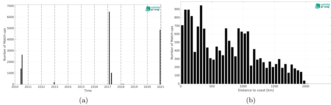
Figure 2: Number of match-ups between TSG (GOSUD-Sailing-ship) and SMOS SSS L4 OI v346 - Weekly (CMEMS-CATDS-LOPS) SSS as a function of time (a) and as function of the distance to coast (b) over the Indian Ocean Pi-MEP region and for the full satellite product period.
